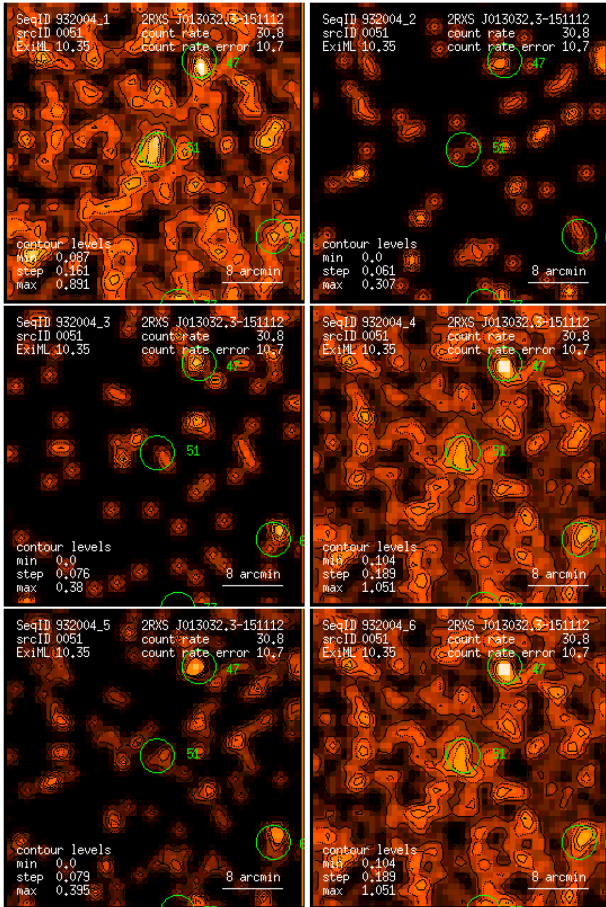
Figure 51: RASS 932004: detection 0051: band rate images, Gaussian filter: (1) PSPC channels 11 – 41, (2) 52 – 90, (3) 91 – 201, (4) 11 – 235, (5) 52 – 201, (6) 11 – 201. Broad band rates in counts/ks. Band rate contour levels in counts/ks/arcmin 2 .
