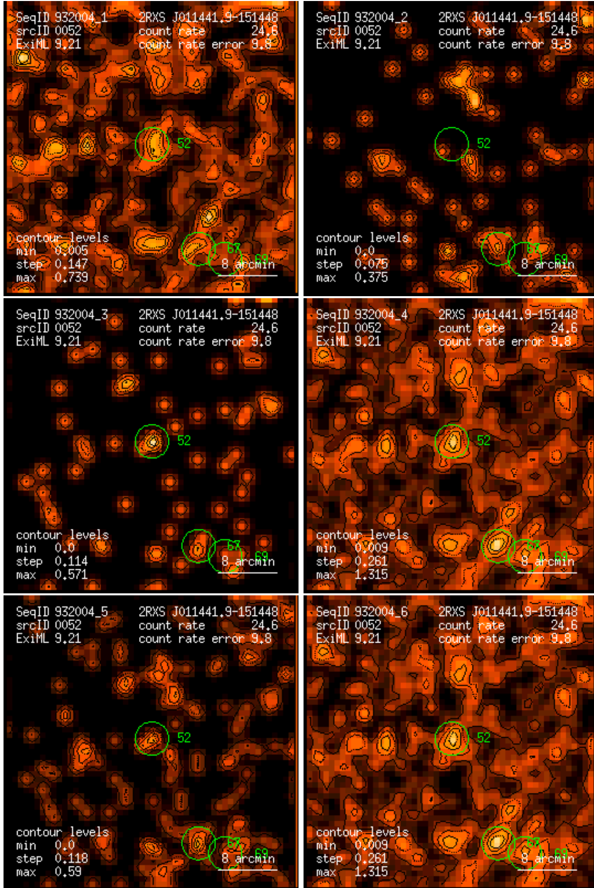
Figure 52: RASS 932004: detection 0052: band rate images, Gaussian filter: (1) PSPC channels 11 – 41, (2) 52 – 90, (3) 91 – 201, (4) 11 – 235, (5) 52 – 201, (6) 11 – 201. Broad band rates in counts/ks. Band rate contour levels in counts/ks/arcmin 2 .
