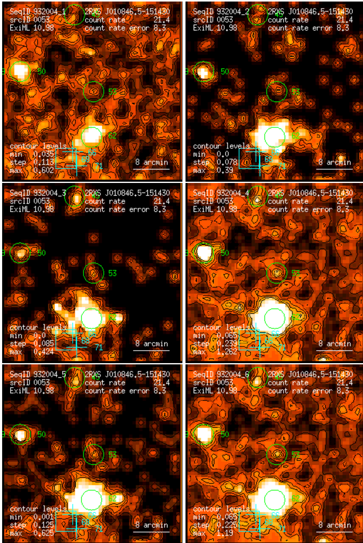
Figure 53: RASS 932004: detection 0053: band rate images, Gaussian filter: (1) PSPC channels 11 – 41, (2) 52 – 90, (3) 91 – 201, (4) 11 – 235, (5) 52 – 201, (6) 11 – 201. Broad band rates in counts/ks. Band rate contour levels in counts/ks/arcmin 2 .
