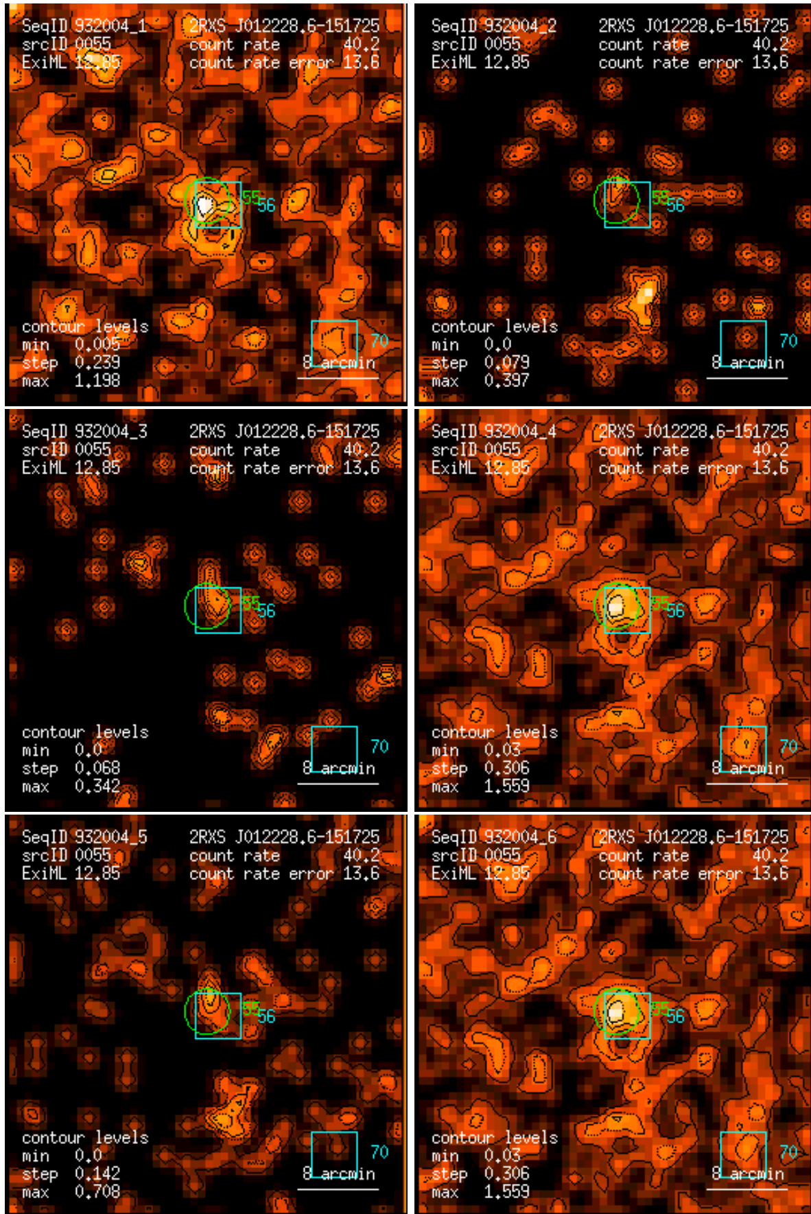
Figure 55: RASS 932004: detection 0055: band rate images, Gaussian filter: (1) PSPC channels 11 – 41, (2) 52 – 90, (3) 91 – 201, (4) 11 – 235, (5) 52 – 201, (6) 11 – 201. Broad band rates in counts/ks. Band rate contour levels in counts/ks/arcmin 2 .
