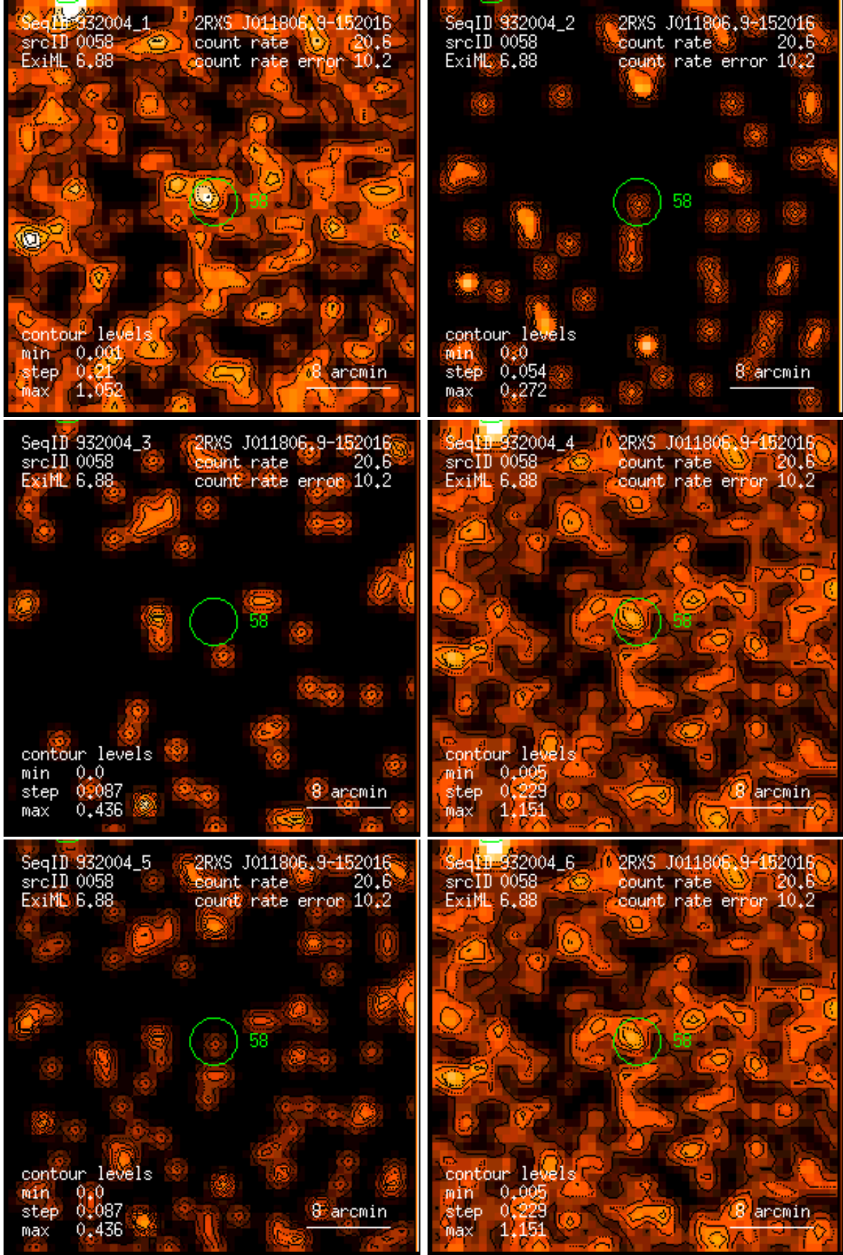
Figure 58: RASS 932004: detection 0058: band rate images, Gaussian filter: (1) PSPC channels 11 – 41, (2) 52 – 90, (3) 91 – 201, (4) 11 – 235, (5) 52 – 201, (6) 11 – 201. Broad band rates in counts/ks. Band rate contour levels in counts/ks/arcmin 2 .
