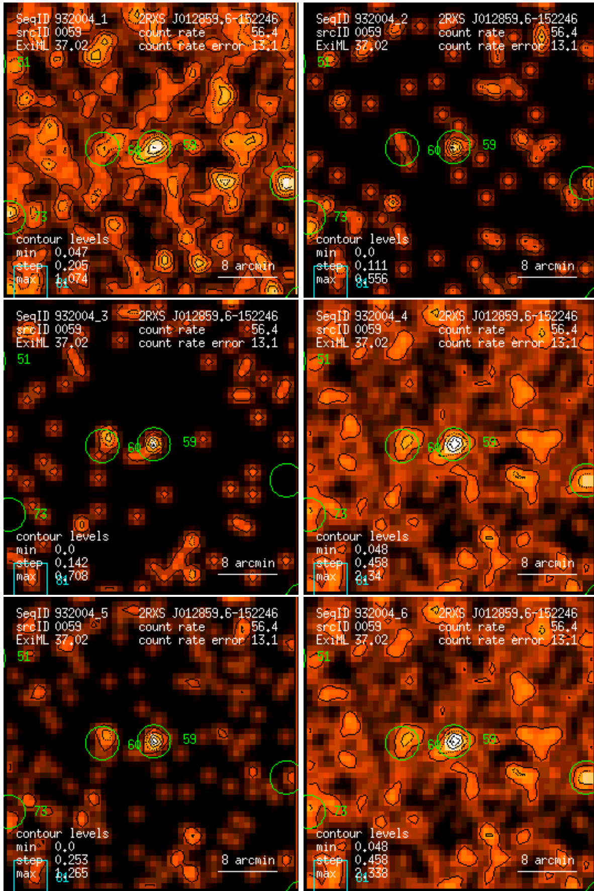
Figure 59: RASS 932004: detection 0059: band rate images, Gaussian filter: (1) PSPC channels 11 – 41, (2) 52 – 90, (3) 91 – 201, (4) 11 – 235, (5) 52 – 201, (6) 11 – 201. Broad band rates in counts/ks. Band rate contour levels in counts/ks/arcmin 2 .
