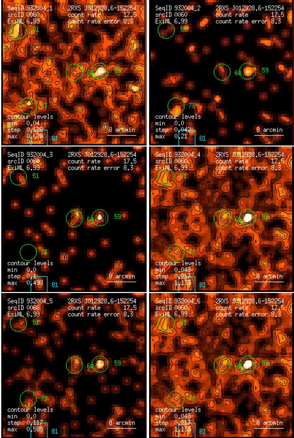
Figure 60: RASS 932004: detection 0060: band rate images, Gaussian filter: (1) PSPC channels 11 – 41, (2) 52 – 90, (3) 91 – 201, (4) 11 – 235, (5) 52 – 201, (6) 11 – 201. Broad band rates in counts/ks. Band rate contour levels in counts/ks/arcmin 2 .
