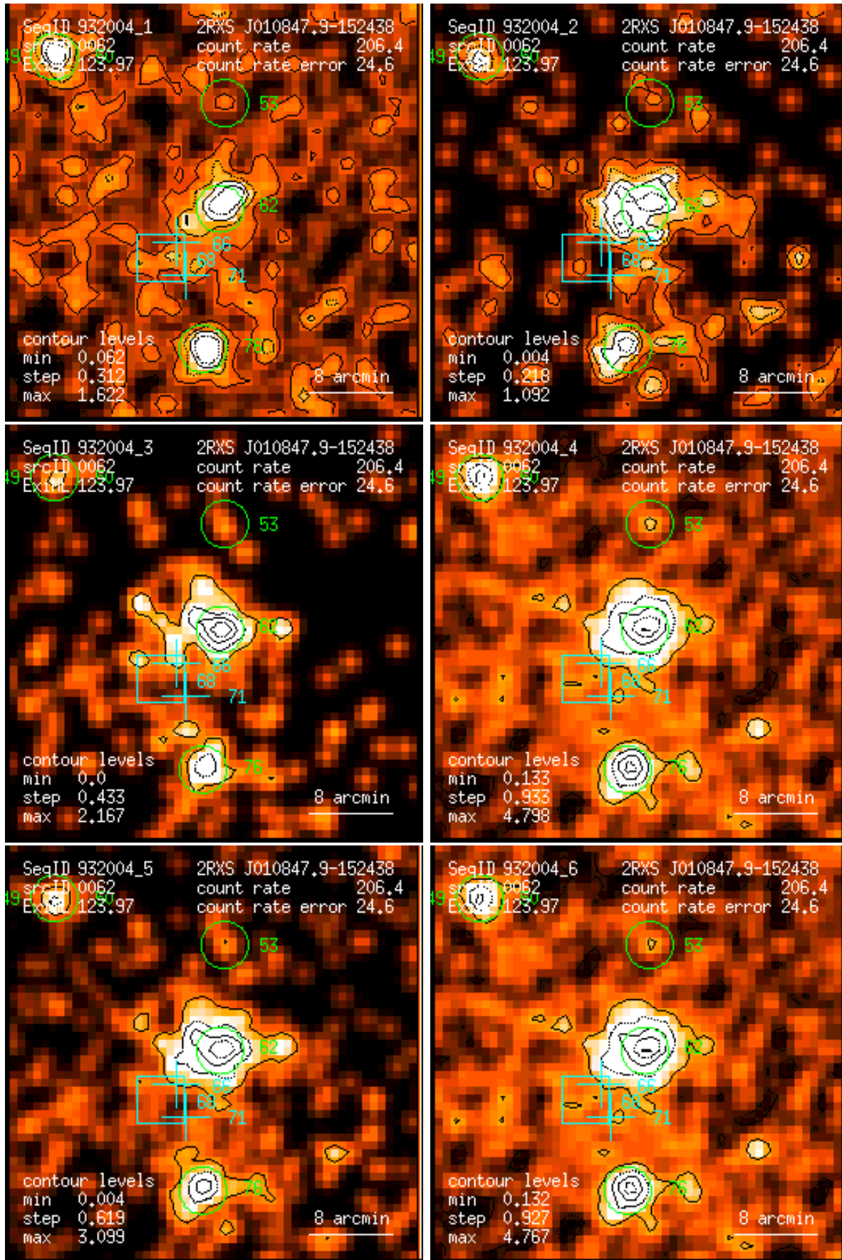
Figure 62: RASS 932004: detection 0062: band rate images, Gaussian filter: (1) PSPC channels 11 – 41, (2) 52 – 90, (3) 91 – 201, (4) 11 – 235, (5) 52 – 201, (6) 11 – 201. Broad band rates in counts/ks. Band rate contour levels in counts/ks/arcmin 2 .
