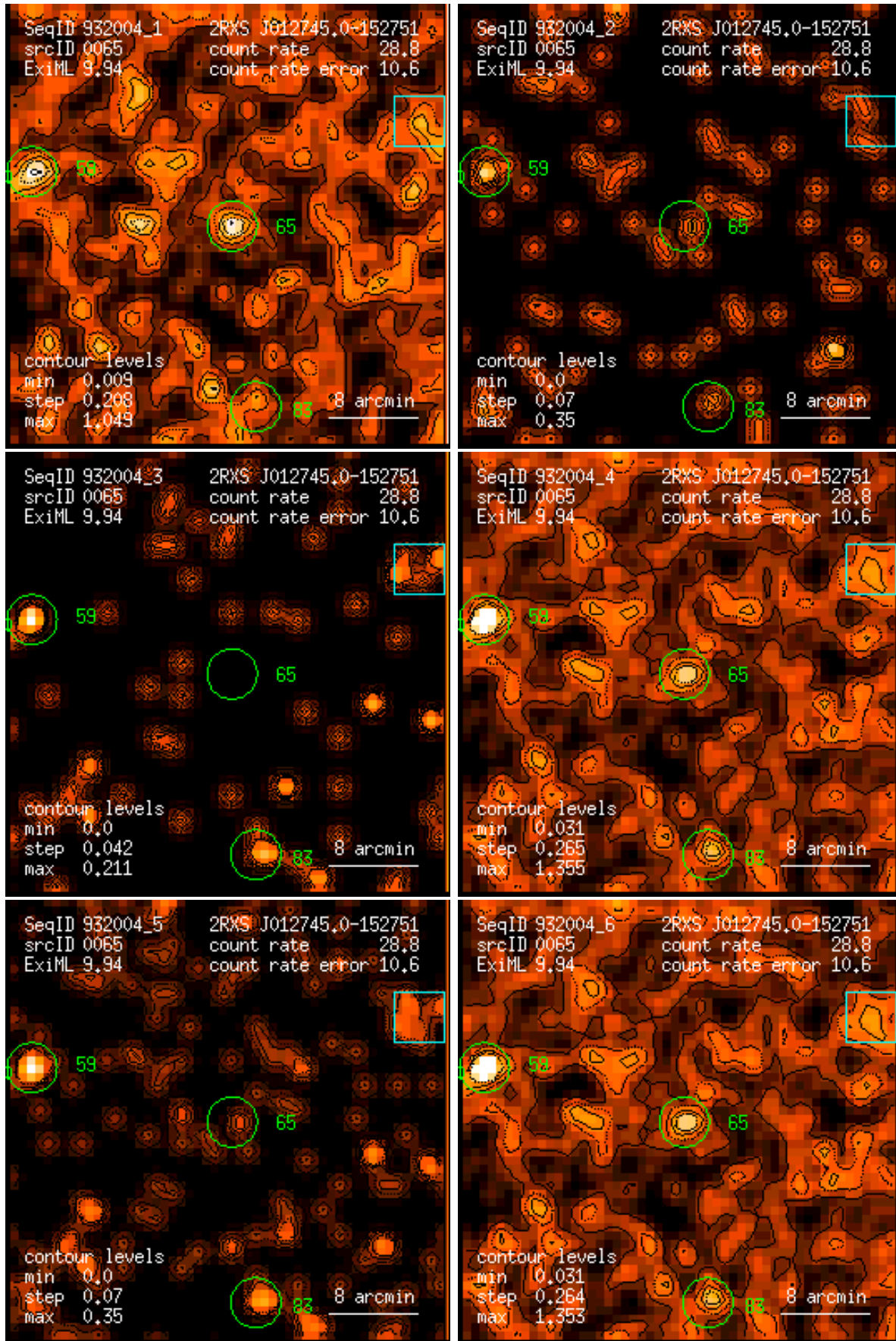
Figure 65: RASS 932004: detection 0065: band rate images, Gaussian filter: (1) PSPC channels 11 – 41, (2) 52 – 90, (3) 91 – 201, (4) 11 – 235, (5) 52 – 201, (6) 11 – 201. Broad band rates in counts/ks. Band rate contour levels in counts/ks/arcmin 2 .
