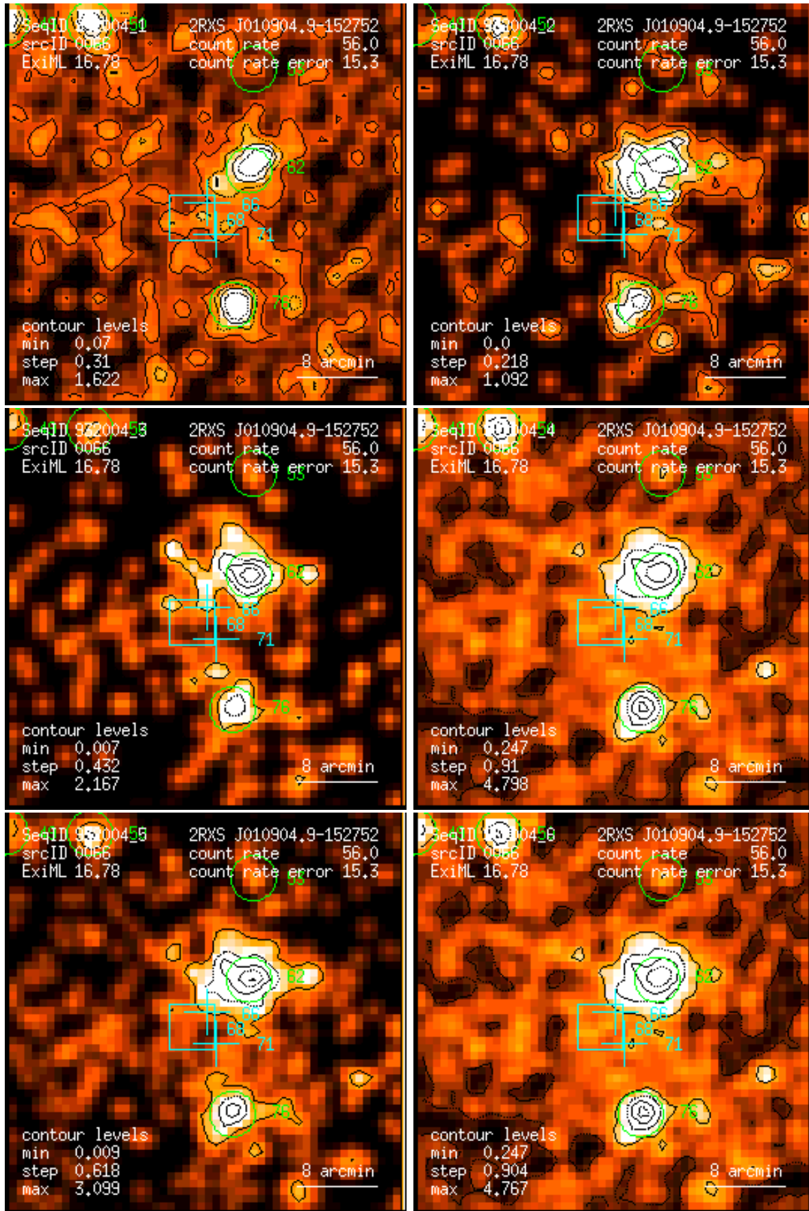
Figure 66: RASS 932004: detection 0066: band rate images, Gaussian filter: (1) PSPC channels 11 – 41, (2) 52 – 90, (3) 91 – 201, (4) 11 – 235, (5) 52 – 201, (6) 11 – 201. Broad band rates in counts/ks. Band rate contour levels in counts/ks/arcmin 2 .
