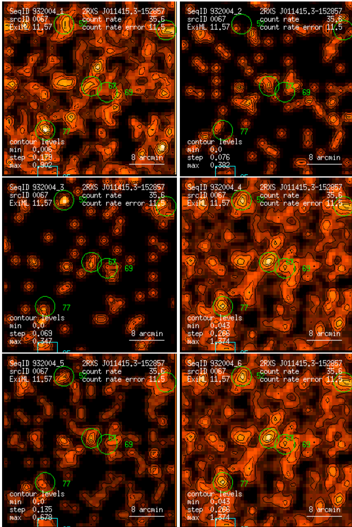
Figure 67: RASS 932004: detection 0067: band rate images, Gaussian filter: (1) PSPC channels 11 – 41, (2) 52 – 90, (3) 91 – 201, (4) 11 – 235, (5) 52 – 201, (6) 11 – 201. Broad band rates in counts/ks. Band rate contour levels in counts/ks/arcmin 2 .
