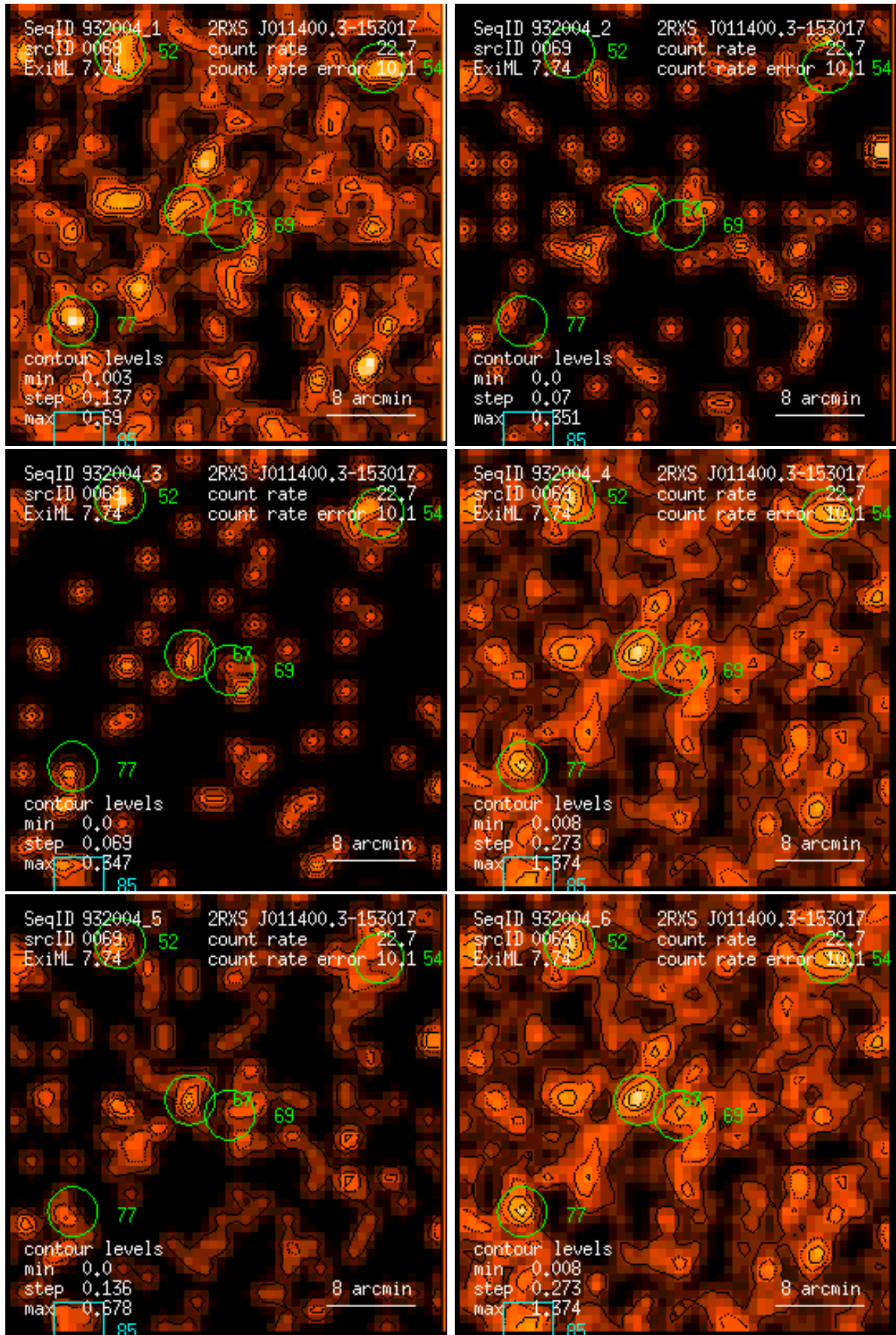
Figure 69: RASS 932004: detection 0069: band rate images, Gaussian filter: (1) PSPC channels 11 – 41, (2) 52 – 90, (3) 91 – 201, (4) 11 – 235, (5) 52 – 201, (6) 11 – 201. Broad band rates in counts/ks. Band rate contour levels in counts/ks/arcmin 2 .
