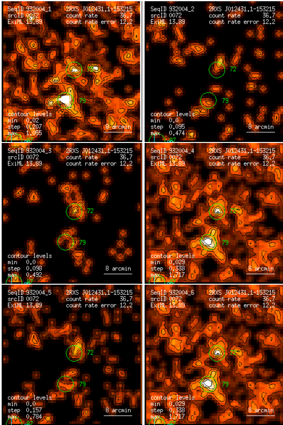
Figure 72: RASS 932004: detection 0072: band rate images, Gaussian filter: (1) PSPC channels 11 – 41, (2) 52 – 90, (3) 91 – 201, (4) 11 – 235, (5) 52 – 201, (6) 11 – 201. Broad band rates in counts/ks. Band rate contour levels in counts/ks/arcmin 2 .
