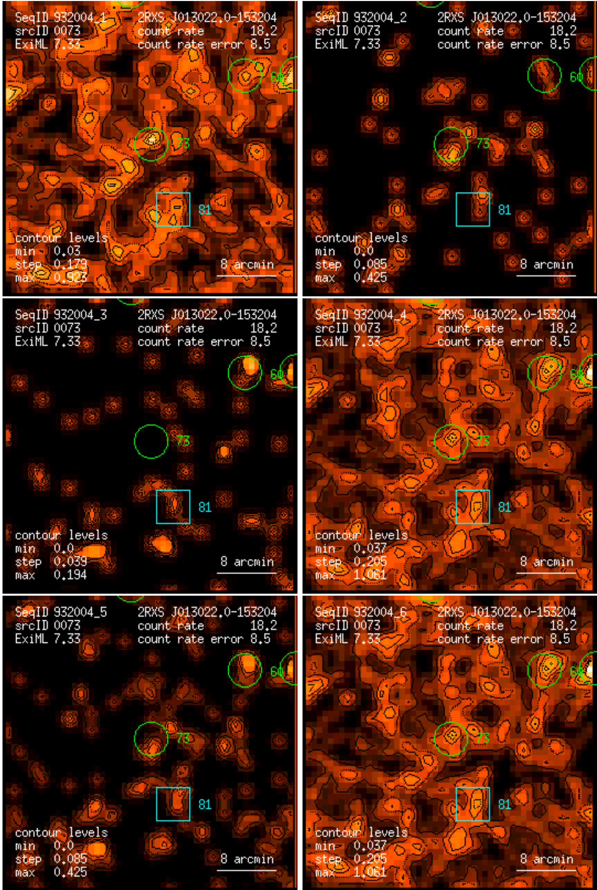
Figure 73: RASS 932004: detection 0073: band rate images, Gaussian filter: (1) PSPC channels 11 – 41, (2) 52 – 90, (3) 91 – 201, (4) 11 – 235, (5) 52 – 201, (6) 11 – 201. Broad band rates in counts/ks. Band rate contour levels in counts/ks/arcmin 2 .
