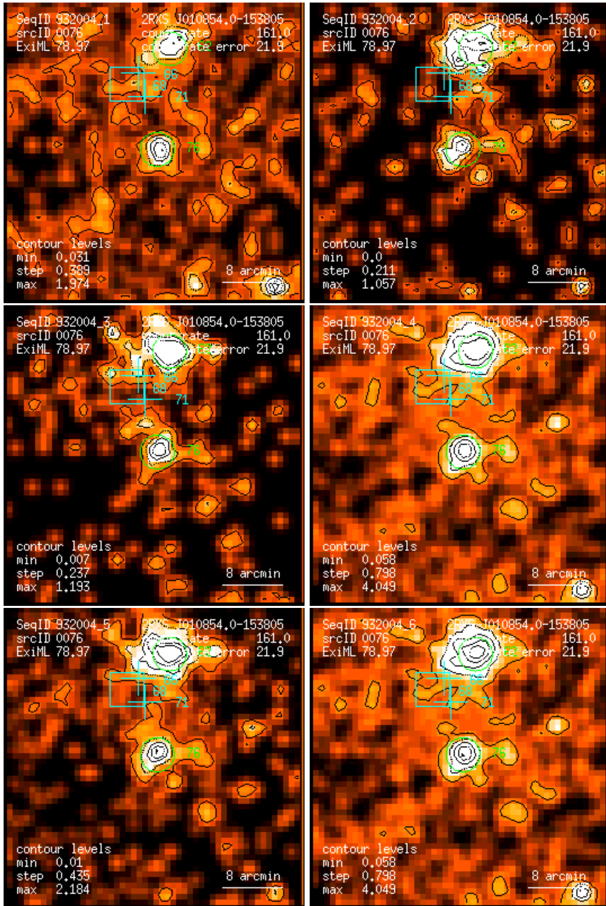
Figure 76: RASS 932004: detection 0076: band rate images, Gaussian filter: (1) PSPC channels 11 – 41, (2) 52 – 90, (3) 91 – 201, (4) 11 – 235, (5) 52 – 201, (6) 11 – 201. Broad band rates in counts/ks. Band rate contour levels in counts/ks/arcmin 2 .
