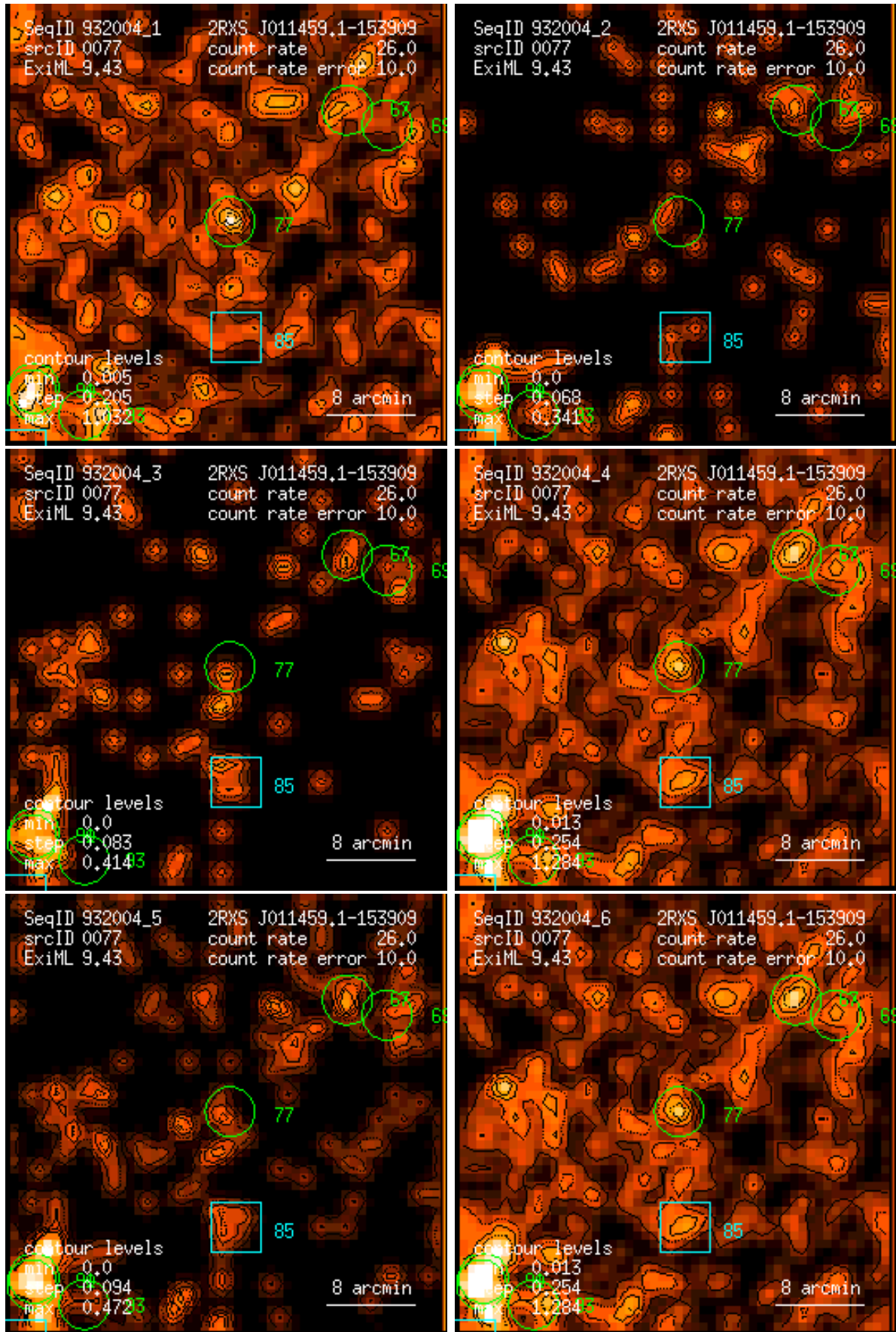
Figure 77: RASS 932004: detection 0077: band rate images, Gaussian filter: (1) PSPC channels 11 – 41, (2) 52 – 90, (3) 91 – 201, (4) 11 – 235, (5) 52 – 201, (6) 11 – 201. Broad band rates in counts/ks. Band rate contour levels in counts/ks/arcmin 2 .
