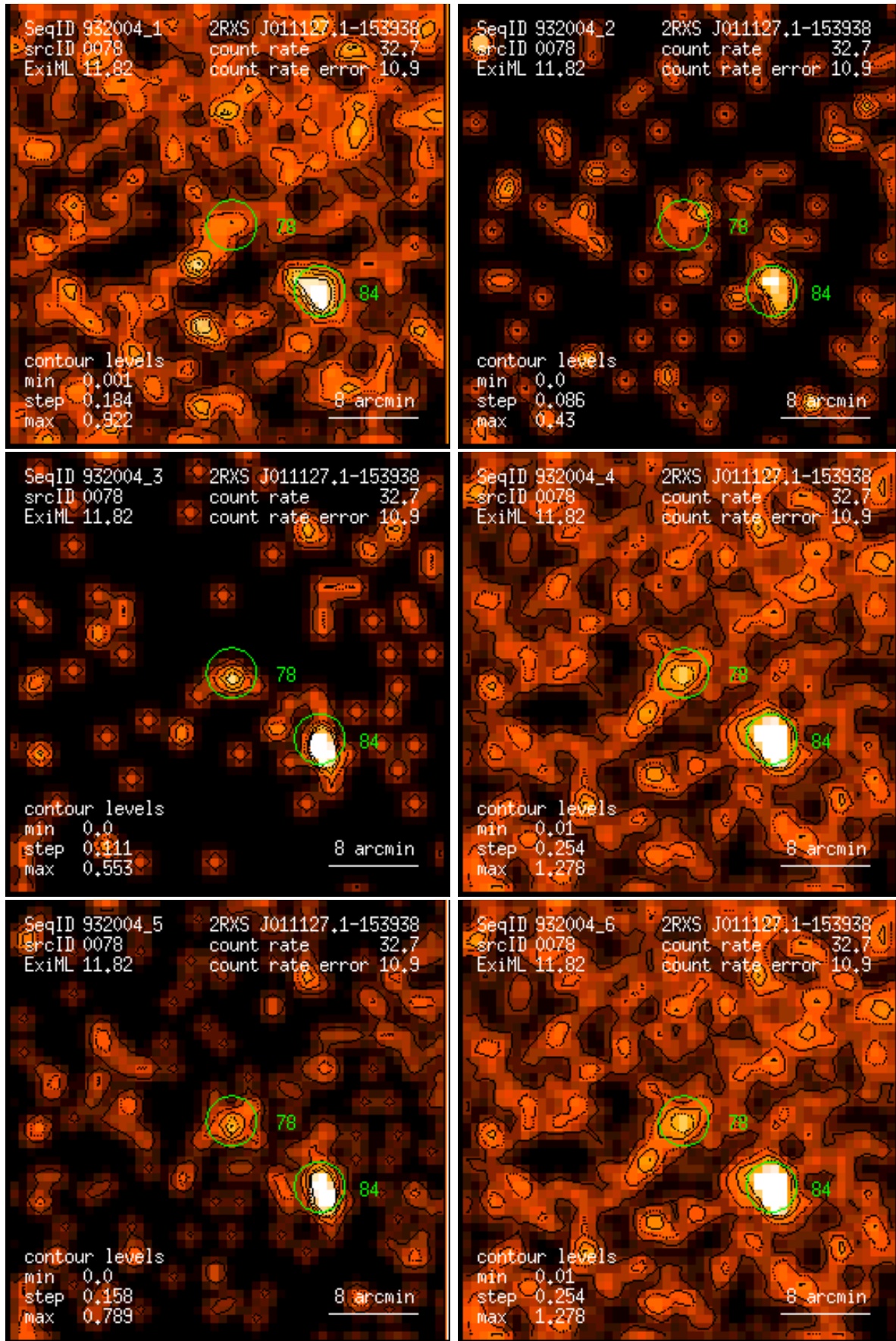
Figure 78: RASS 932004: detection 0078: band rate images, Gaussian filter: (1) PSPC channels 11 – 41, (2) 52 – 90, (3) 91 – 201, (4) 11 – 235, (5) 52 – 201, (6) 11 – 201. Broad band rates in counts/ks. Band rate contour levels in counts/ks/arcmin 2 .
