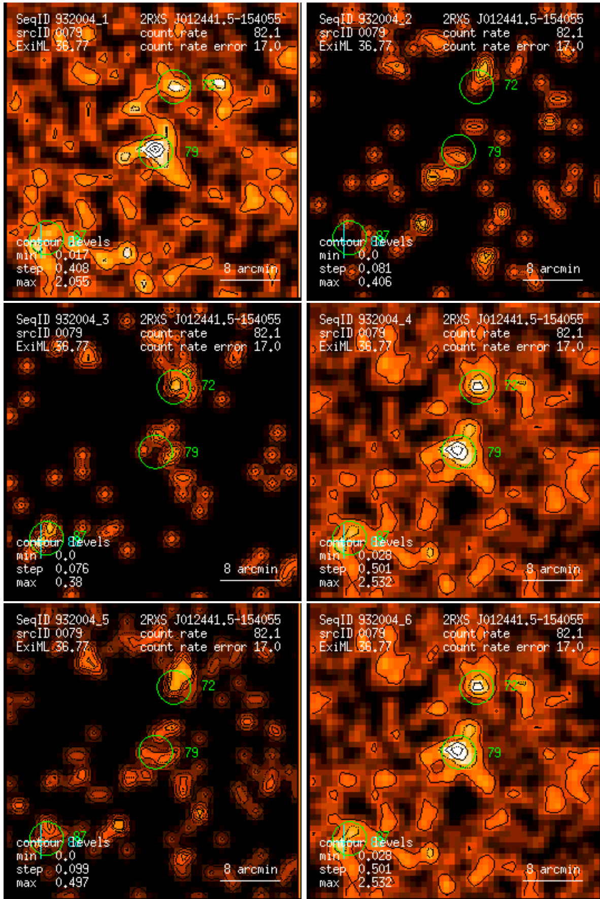
Figure 79: RASS 932004: detection 0079: band rate images, Gaussian filter: (1) PSPC channels 11 – 41, (2) 52 – 90, (3) 91 – 201, (4) 11 – 235, (5) 52 – 201, (6) 11 – 201. Broad band rates in counts/ks. Band rate contour levels in counts/ks/arcmin 2 .
