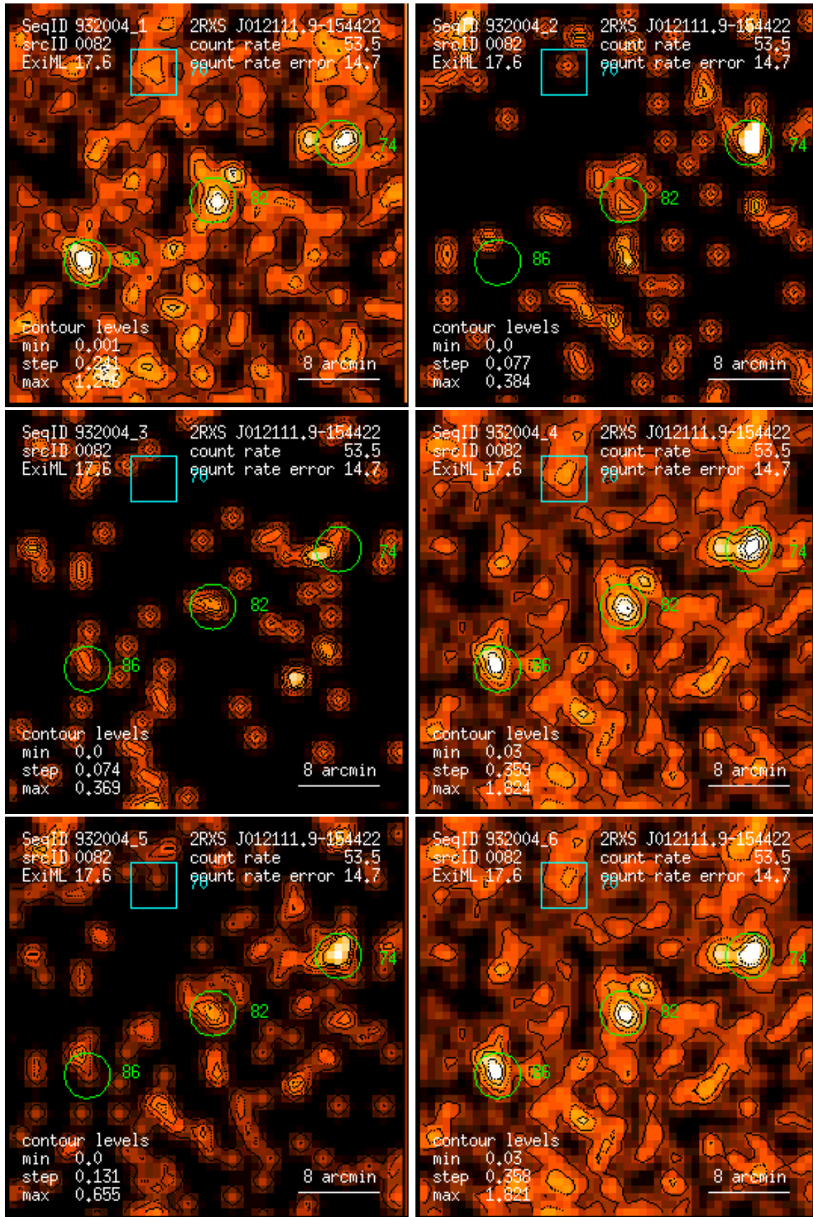
Figure 82: RASS 932004: detection 0082: band rate images, Gaussian filter: (1) PSPC channels 11 – 41, (2) 52 – 90, (3) 91 – 201, (4) 11 – 235, (5) 52 – 201, (6) 11 – 201. Broad band rates in counts/ks. Band rate contour levels in counts/ks/arcmin 2 .
