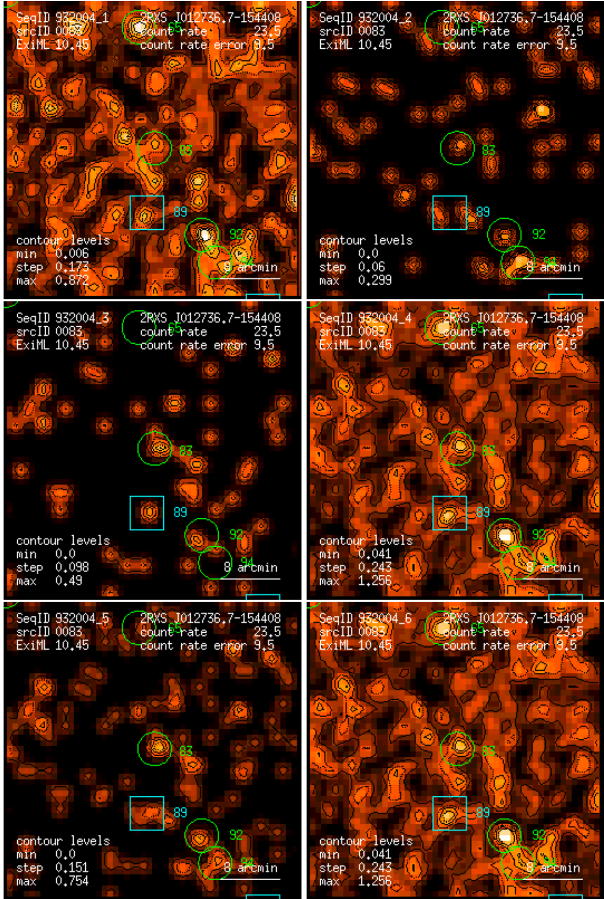
Figure 83: RASS 932004: detection 0083: band rate images, Gaussian filter: (1) PSPC channels 11 – 41, (2) 52 – 90, (3) 91 – 201, (4) 11 – 235, (5) 52 – 201, (6) 11 – 201. Broad band rates in counts/ks. Band rate contour levels in counts/ks/arcmin 2 .
