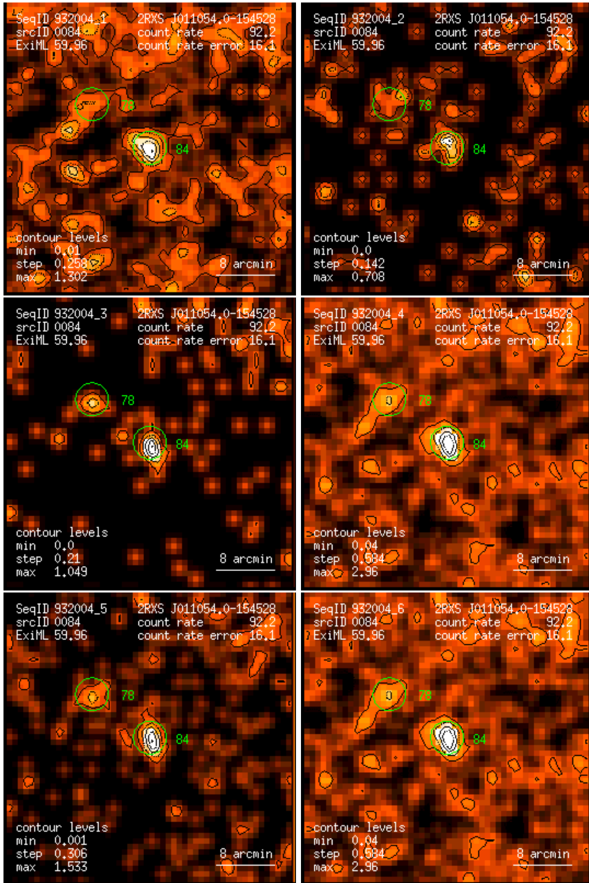
Figure 84: RASS 932004: detection 0084: band rate images, Gaussian filter: (1) PSPC channels 11 – 41, (2) 52 – 90, (3) 91 – 201, (4) 11 – 235, (5) 52 – 201, (6) 11 – 201. Broad band rates in counts/ks. Band rate contour levels in counts/ks/arcmin 2 .
