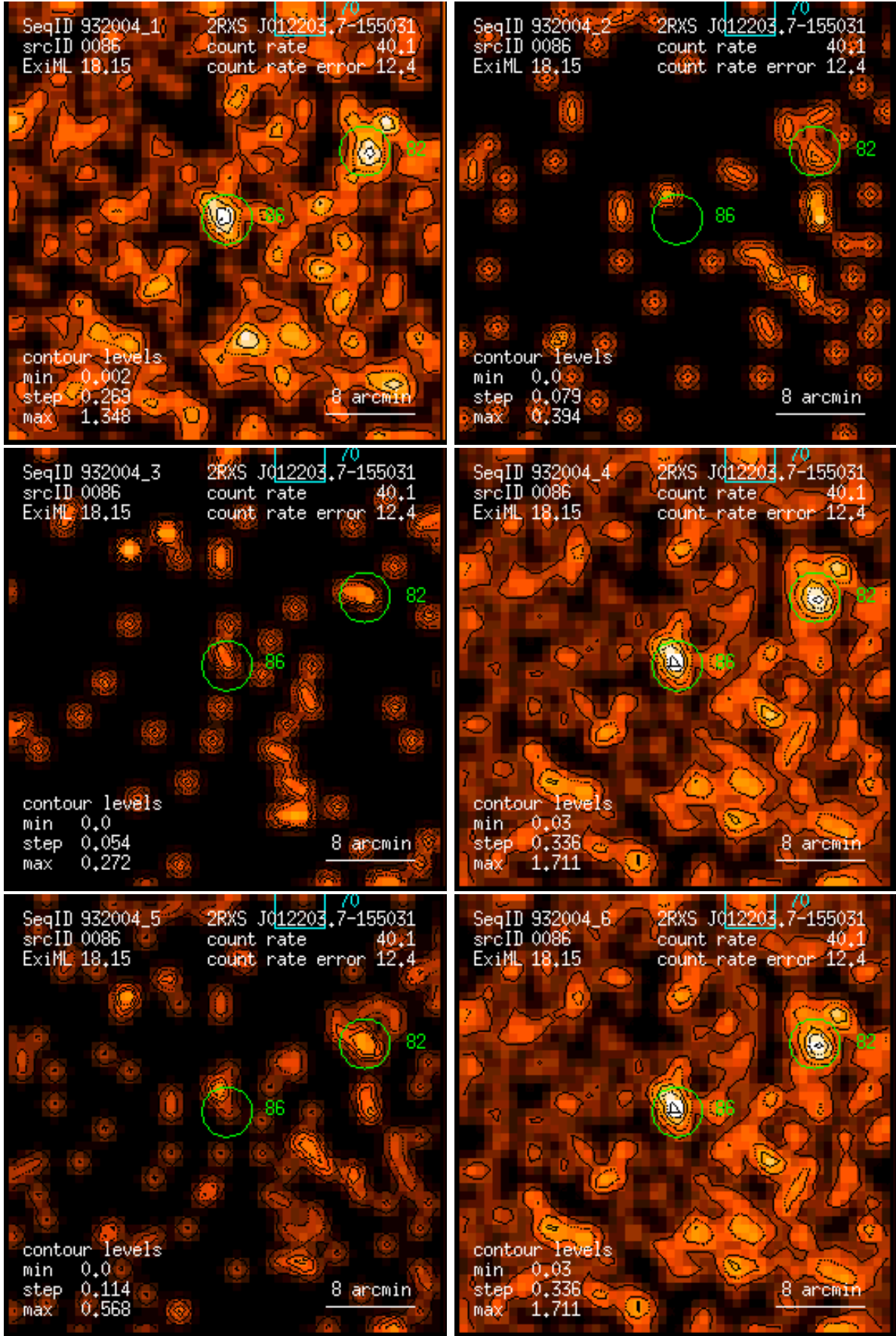
Figure 86: RASS 932004: detection 0086: band rate images, Gaussian filter: (1) PSPC channels 11 – 41, (2) 52 – 90, (3) 91 – 201, (4) 11 – 235, (5) 52 – 201, (6) 11 – 201. Broad band rates in counts/ks. Band rate contour levels in counts/ks/arcmin 2 .
