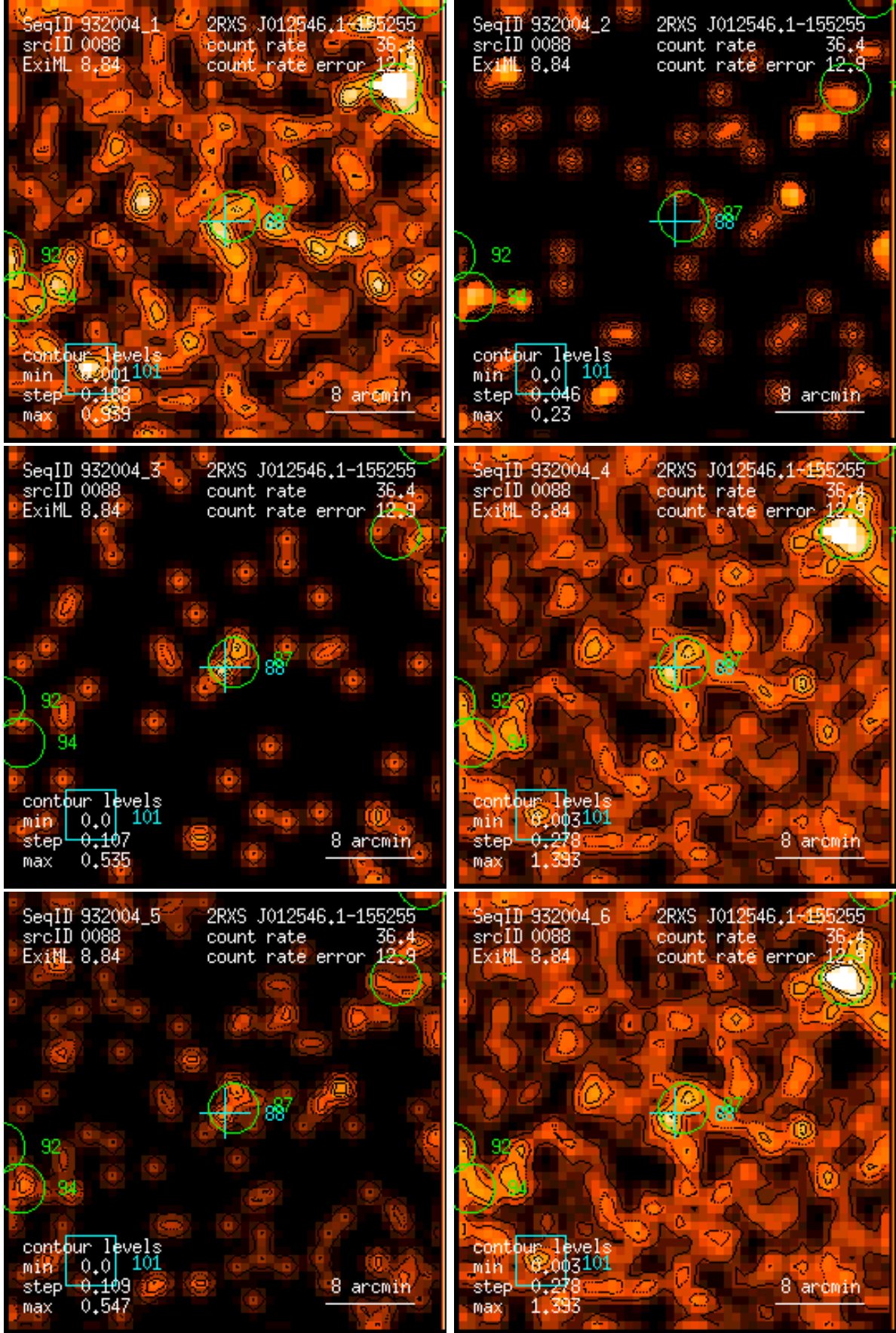
Figure 88: RASS 932004: detection 0088: band rate images, Gaussian filter: (1) PSPC channels 11 – 41, (2) 52 – 90, (3) 91 – 201, (4) 11 – 235, (5) 52 – 201, (6) 11 – 201. Broad band rates in counts/ks. Band rate contour levels in counts/ks/arcmin 2 .
