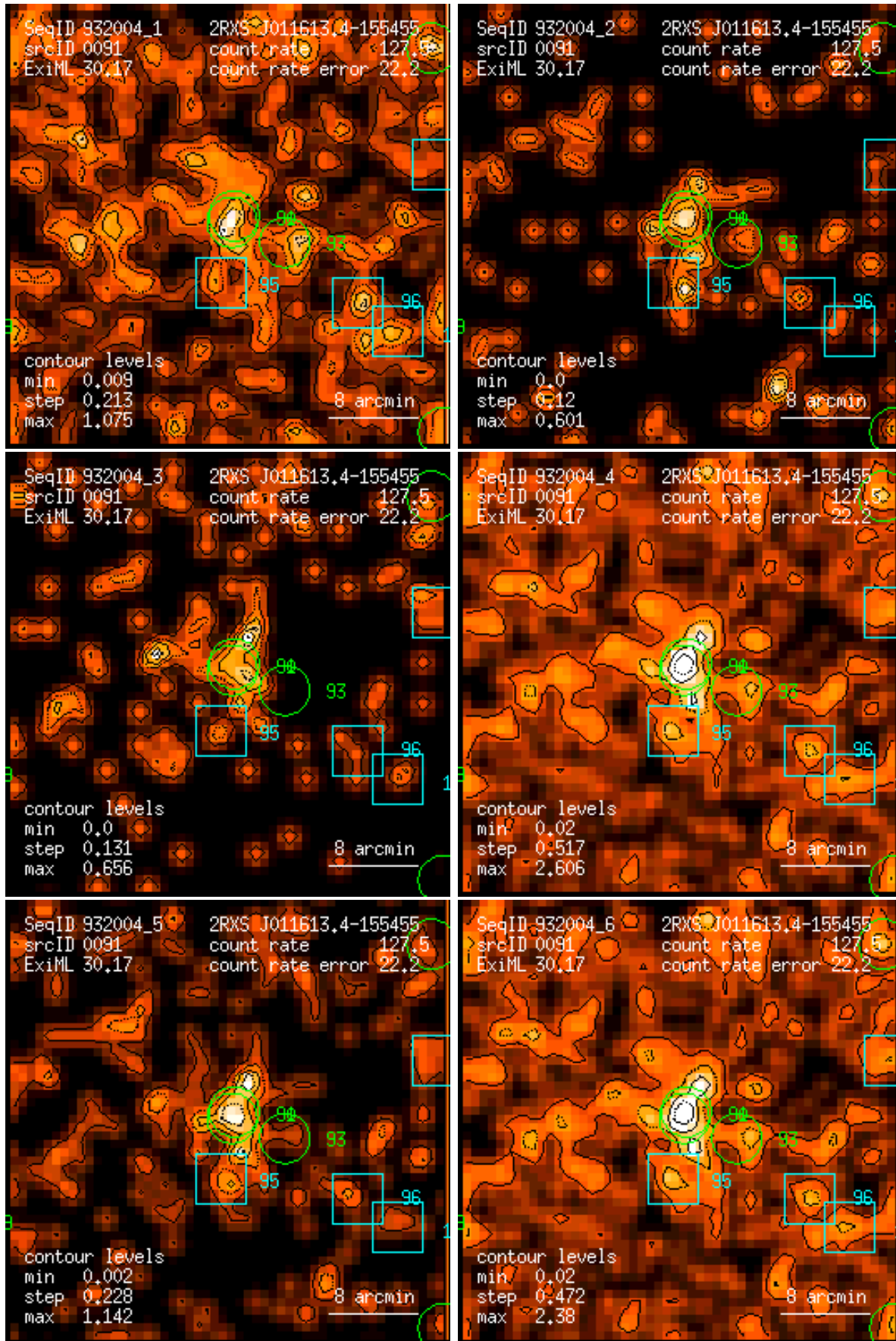
Figure 91: RASS 932004: detection 0091: band rate images, Gaussian filter: (1) PSPC channels 11 – 41, (2) 52 – 90, (3) 91 – 201, (4) 11 – 235, (5) 52 – 201, (6) 11 – 201. Broad band rates in counts/ks. Band rate contour levels in counts/ks/arcmin 2 .
