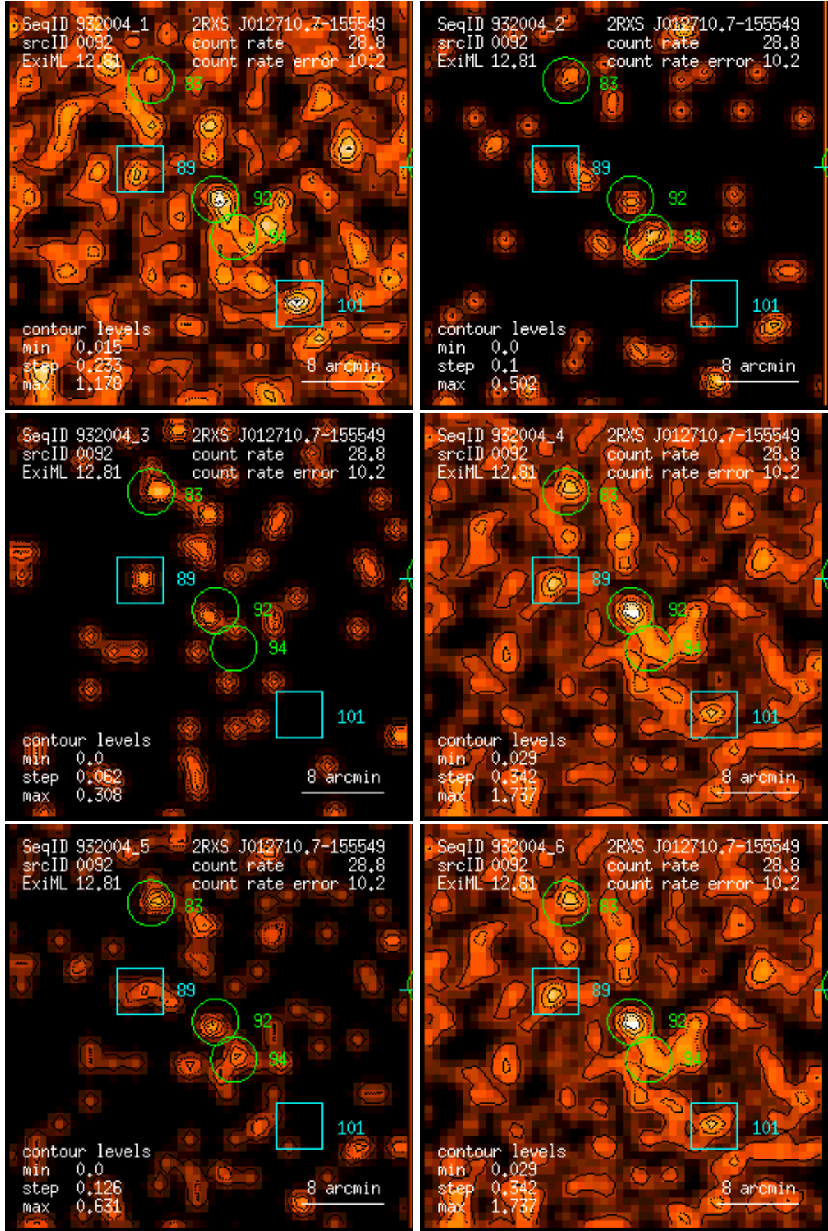
Figure 92: RASS 932004: detection 0092: band rate images, Gaussian filter: (1) PSPC channels 11 – 41, (2) 52 – 90, (3) 91 – 201, (4) 11 – 235, (5) 52 – 201, (6) 11 – 201. Broad band rates in counts/ks. Band rate contour levels in counts/ks/arcmin 2 .
