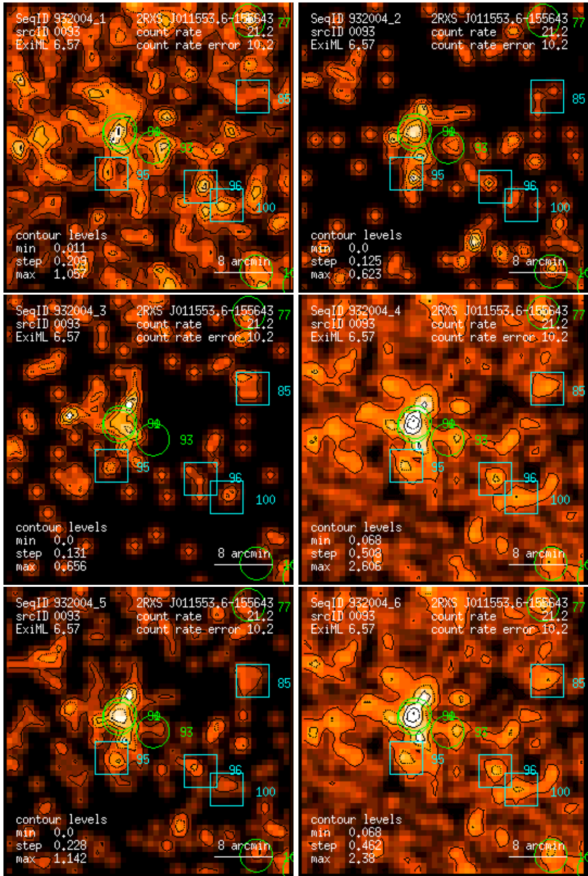
Figure 93: RASS 932004: detection 0093: band rate images, Gaussian filter: (1) PSPC channels 11 – 41, (2) 52 – 90, (3) 91 – 201, (4) 11 – 235, (5) 52 – 201, (6) 11 – 201. Broad band rates in counts/ks. Band rate contour levels in counts/ks/arcmin 2 .
