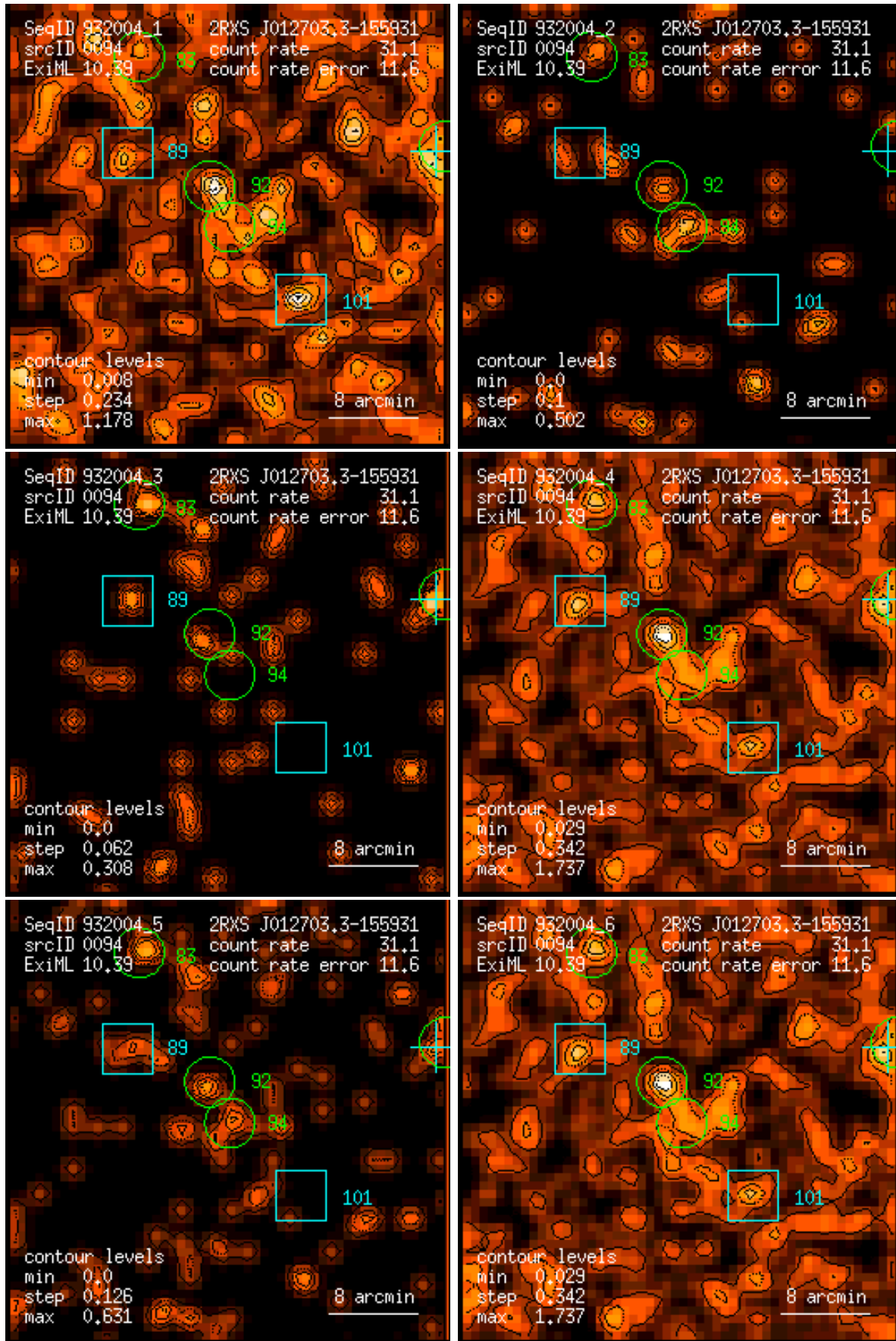
Figure 94: RASS 932004: detection 0094: band rate images, Gaussian filter: (1) PSPC channels 11 – 41, (2) 52 – 90, (3) 91 – 201, (4) 11 – 235, (5) 52 – 201, (6) 11 – 201. Broad band rates in counts/ks. Band rate contour levels in counts/ks/arcmin 2 .
