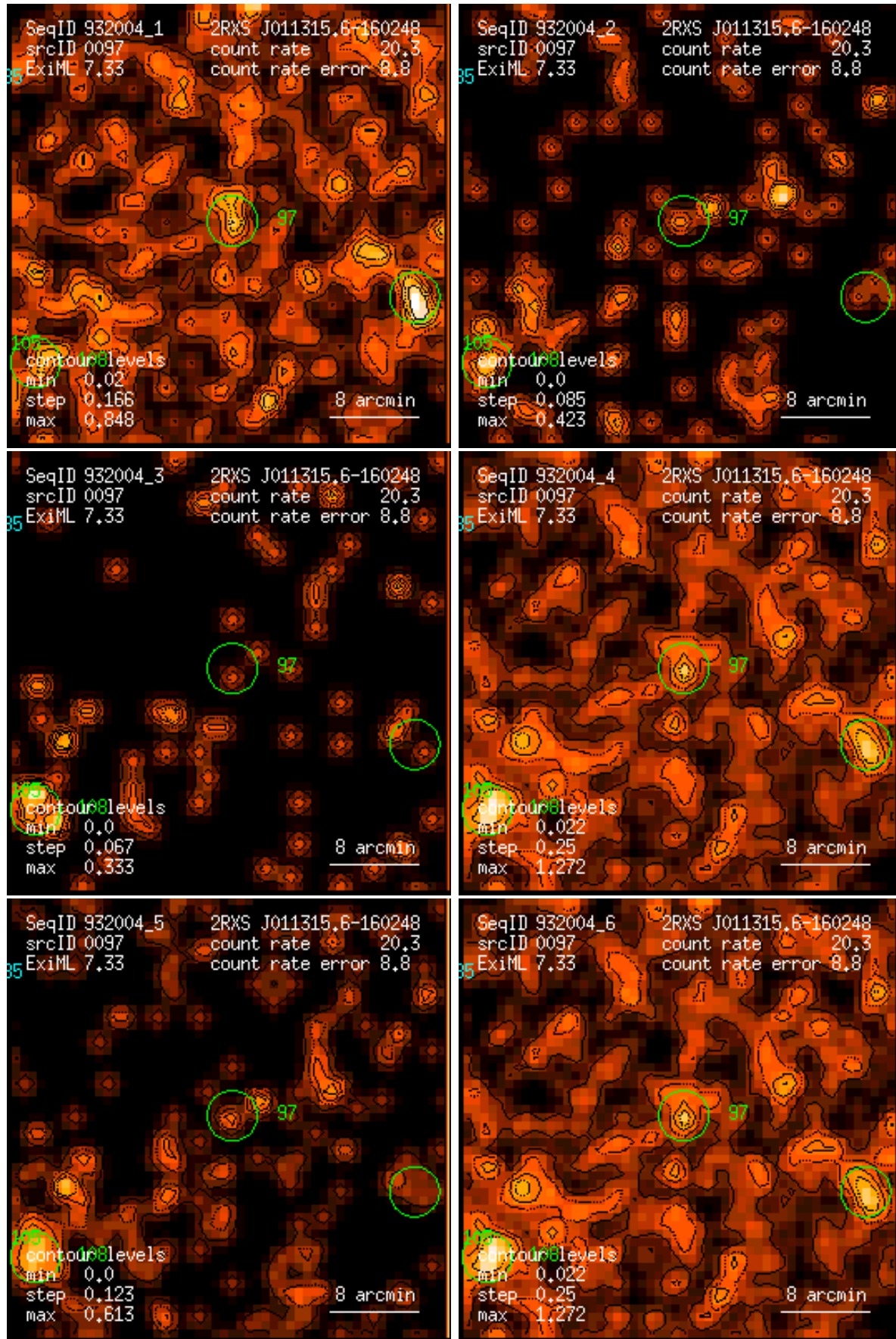
Figure 97: RASS 932004: detection 0097: band rate images, Gaussian filter: (1) PSPC channels 11 – 41, (2) 52 – 90, (3) 91 – 201, (4) 11 – 235, (5) 52 – 201, (6) 11 – 201. Broad band rates in counts/ks. Band rate contour levels in counts/ks/arcmin 2 .
