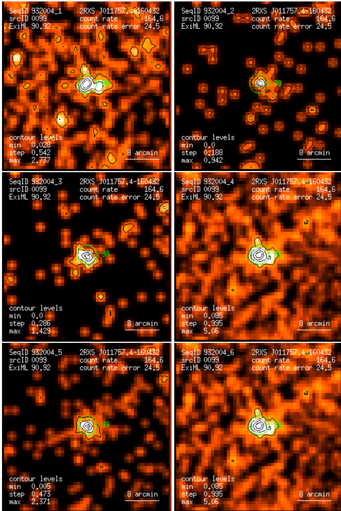
Figure 99: RASS 932004: detection 0099: band rate images, Gaussian filter: (1) PSPC channels 11 – 41, (2) 52 – 90, (3) 91 – 201, (4) 11 – 235, (5) 52 – 201, (6) 11 – 201. Broad band rates in counts/ks. Band rate contour levels in counts/ks/arcmin 2 .
