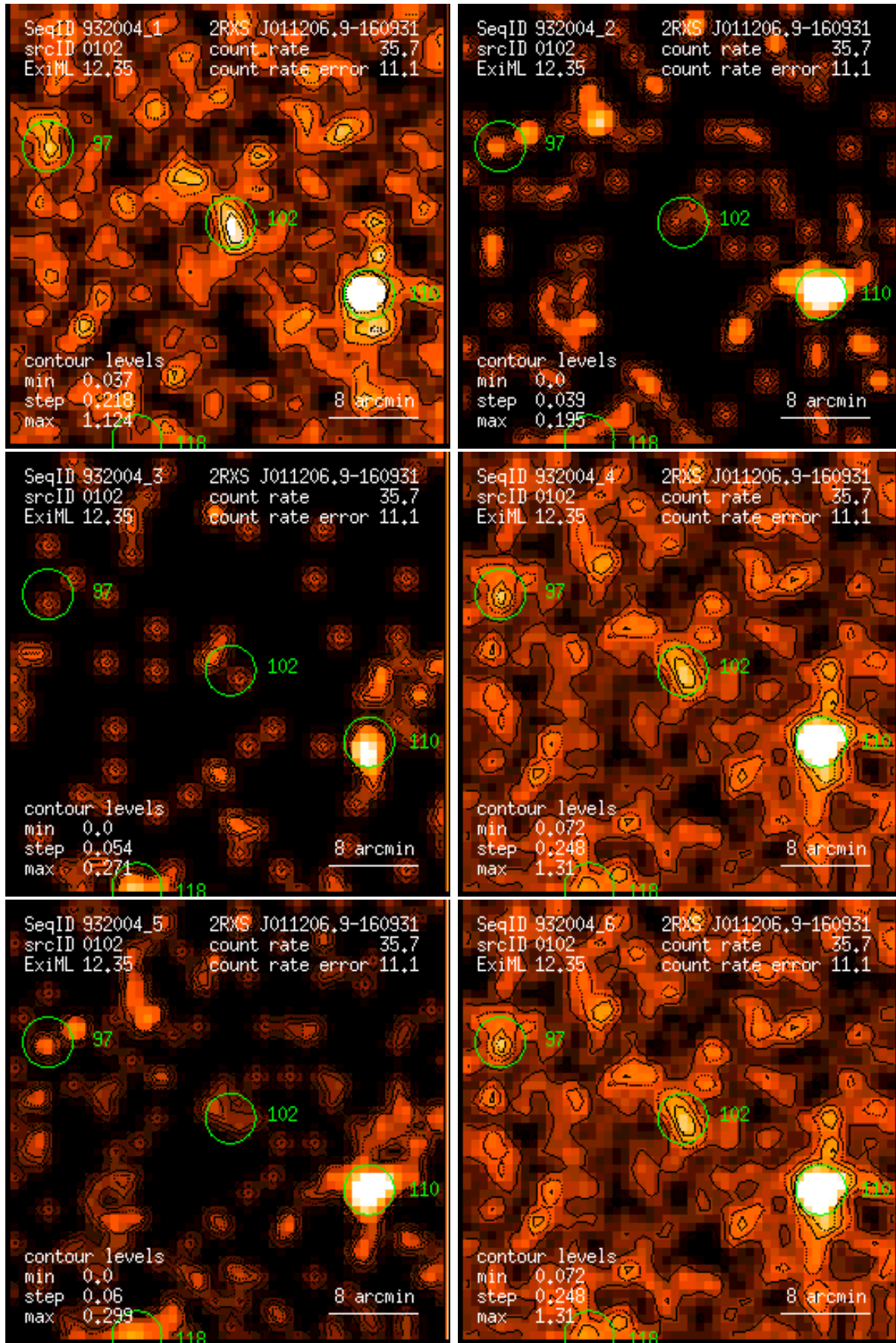
Figure 102: RASS 932004: detection 0102: band rate images, Gaussian filter: (1) PSPC channels 11 – 41, (2) 52 – 90, (3) 91 – 201, (4) 11 – 235, (5) 52 – 201, (6) 11 – 201. Broad band rates in counts/ks. Band rate contour levels in counts/ks/arcmin 2 .
