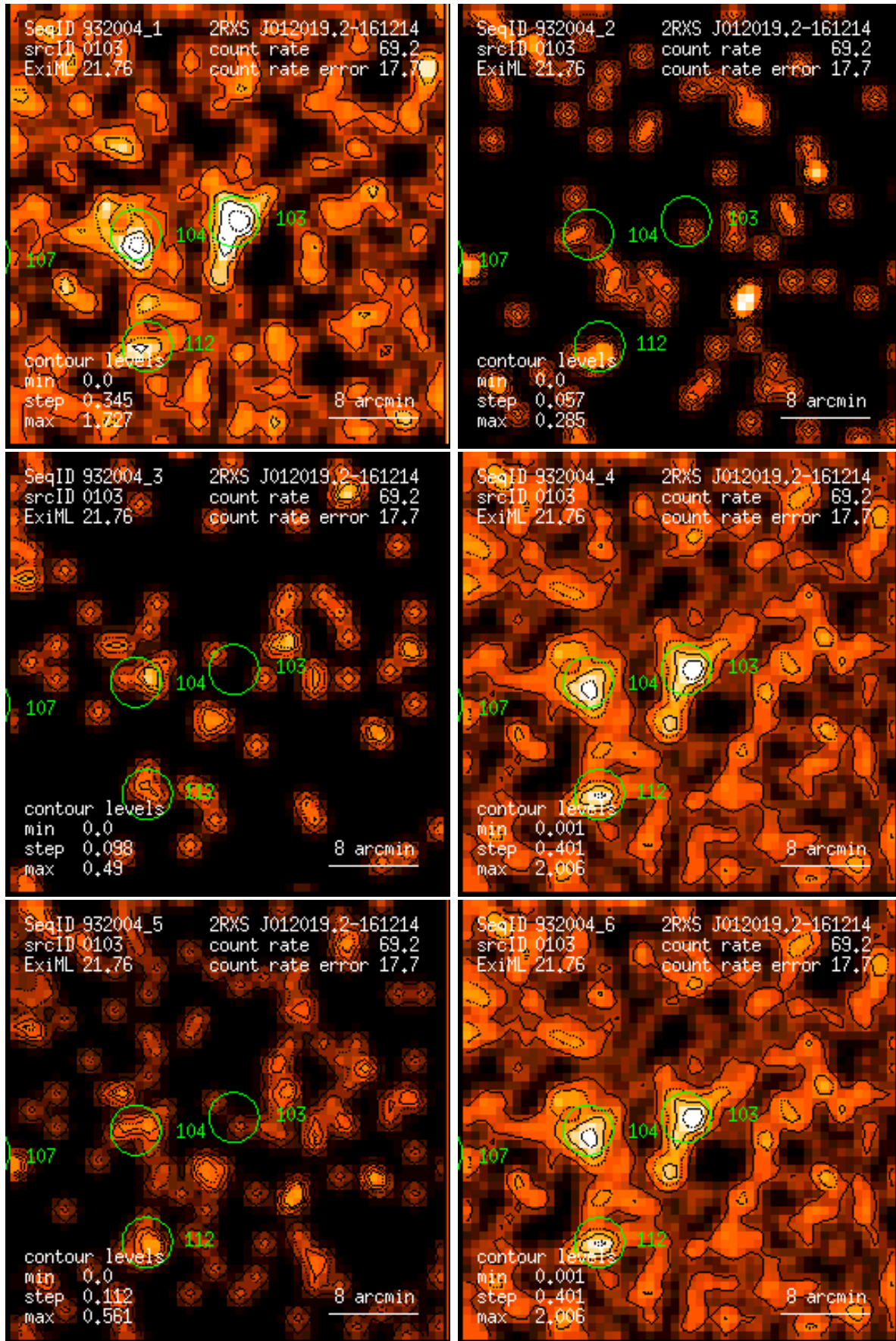
Figure 103: RASS 932004: detection 0103: band rate images, Gaussian filter: (1) PSPC channels 11 – 41, (2) 52 – 90, (3) 91 – 201, (4) 11 – 235, (5) 52 – 201, (6) 11 – 201. Broad band rates in counts/ks. Band rate contour levels in counts/ks/arcmin 2 .
