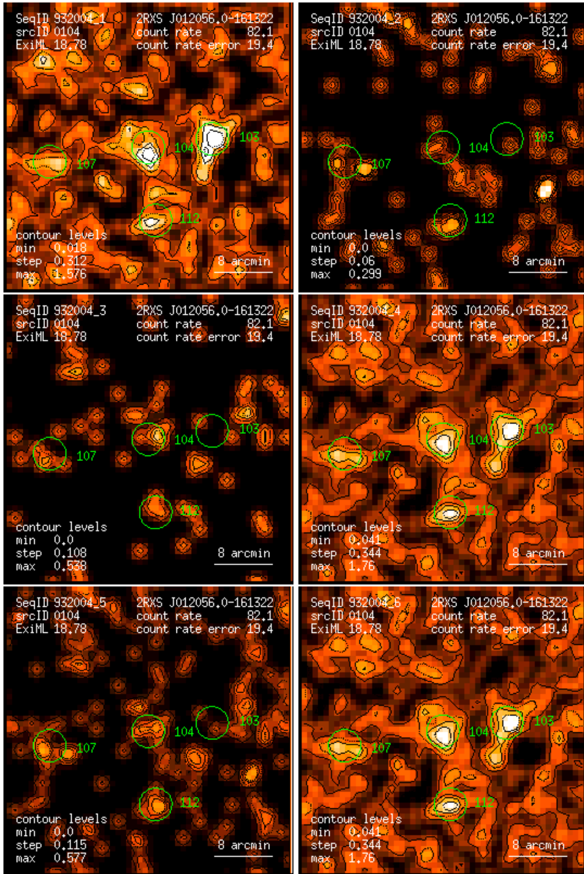
Figure 104: RASS 932004: detection 0104: band rate images, Gaussian filter: (1) PSPC channels 11 – 41, (2) 52 – 90, (3) 91 – 201, (4) 11 – 235, (5) 52 – 201, (6) 11 – 201. Broad band rates in counts/ks. Band rate contour levels in counts/ks/arcmin 2 .
