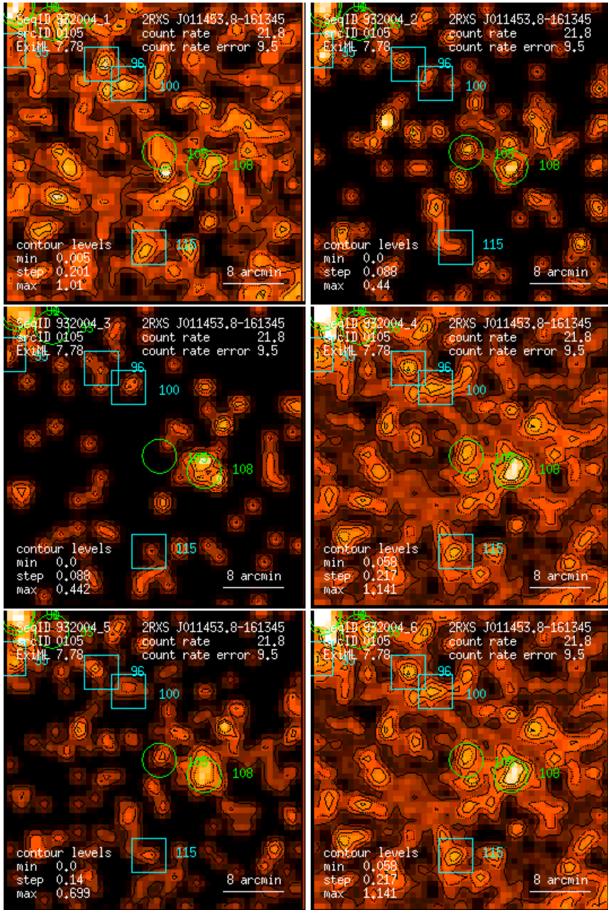
Figure 105: RASS 932004: detection 0105: band rate images, Gaussian filter: (1) PSPC channels 11 – 41, (2) 52 – 90, (3) 91 – 201, (4) 11 – 235, (5) 52 – 201, (6) 11 – 201. Broad band rates in counts/ks. Band rate contour levels in counts/ks/arcmin 2 .
