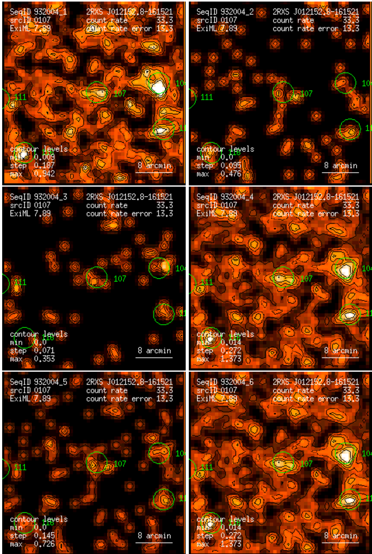
Figure 107: RASS 932004: detection 0107: band rate images, Gaussian filter: (1) PSPC channels 11 – 41, (2) 52 – 90, (3) 91 – 201, (4) 11 – 235, (5) 52 – 201, (6) 11 – 201. Broad band rates in counts/ks. Band rate contour levels in counts/ks/arcmin 2 .
