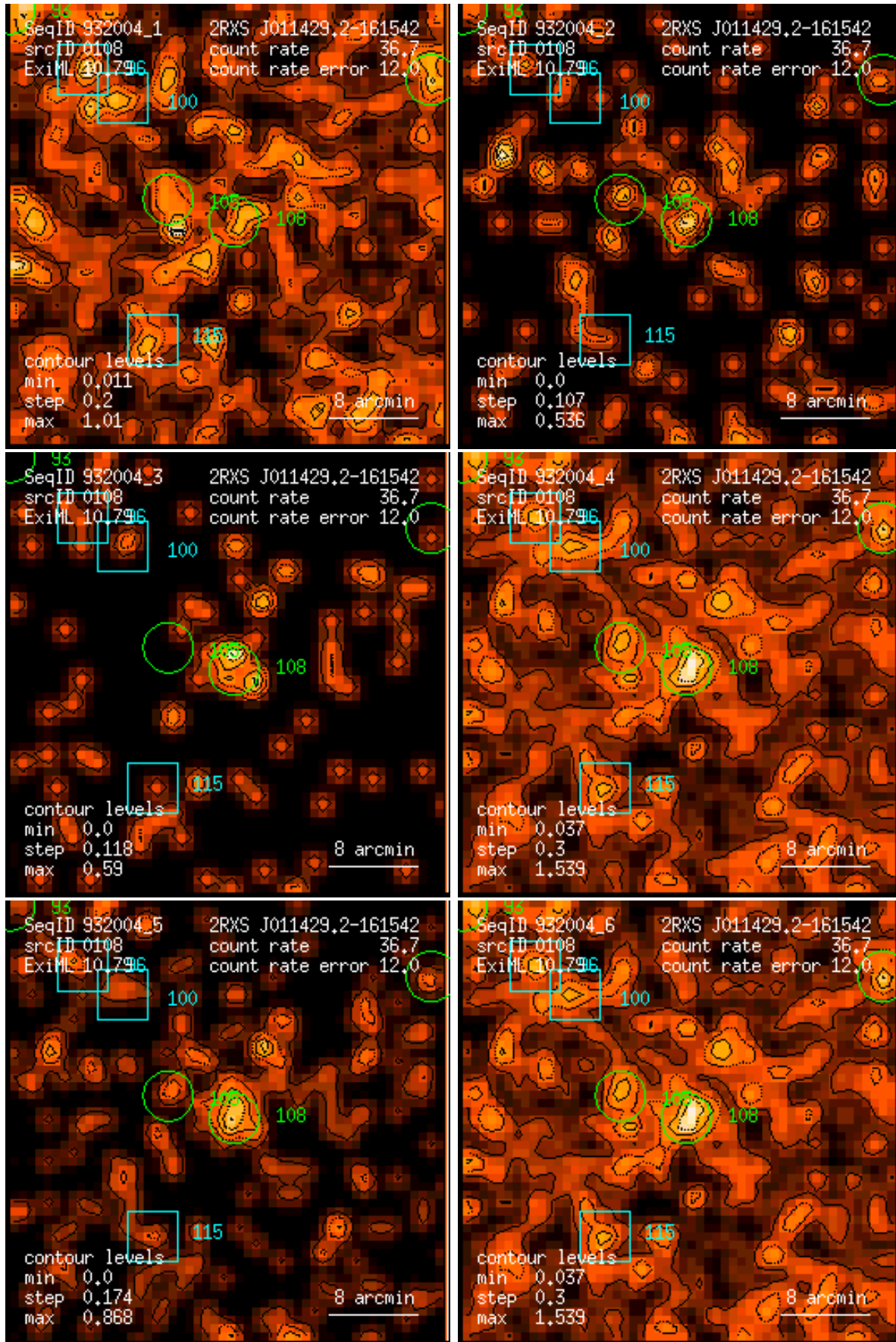
Figure 108: RASS 932004: detection 0108: band rate images, Gaussian filter: (1) PSPC channels 11 – 41, (2) 52 – 90, (3) 91 – 201, (4) 11 – 235, (5) 52 – 201, (6) 11 – 201. Broad band rates in counts/ks. Band rate contour levels in counts/ks/arcmin 2 .
