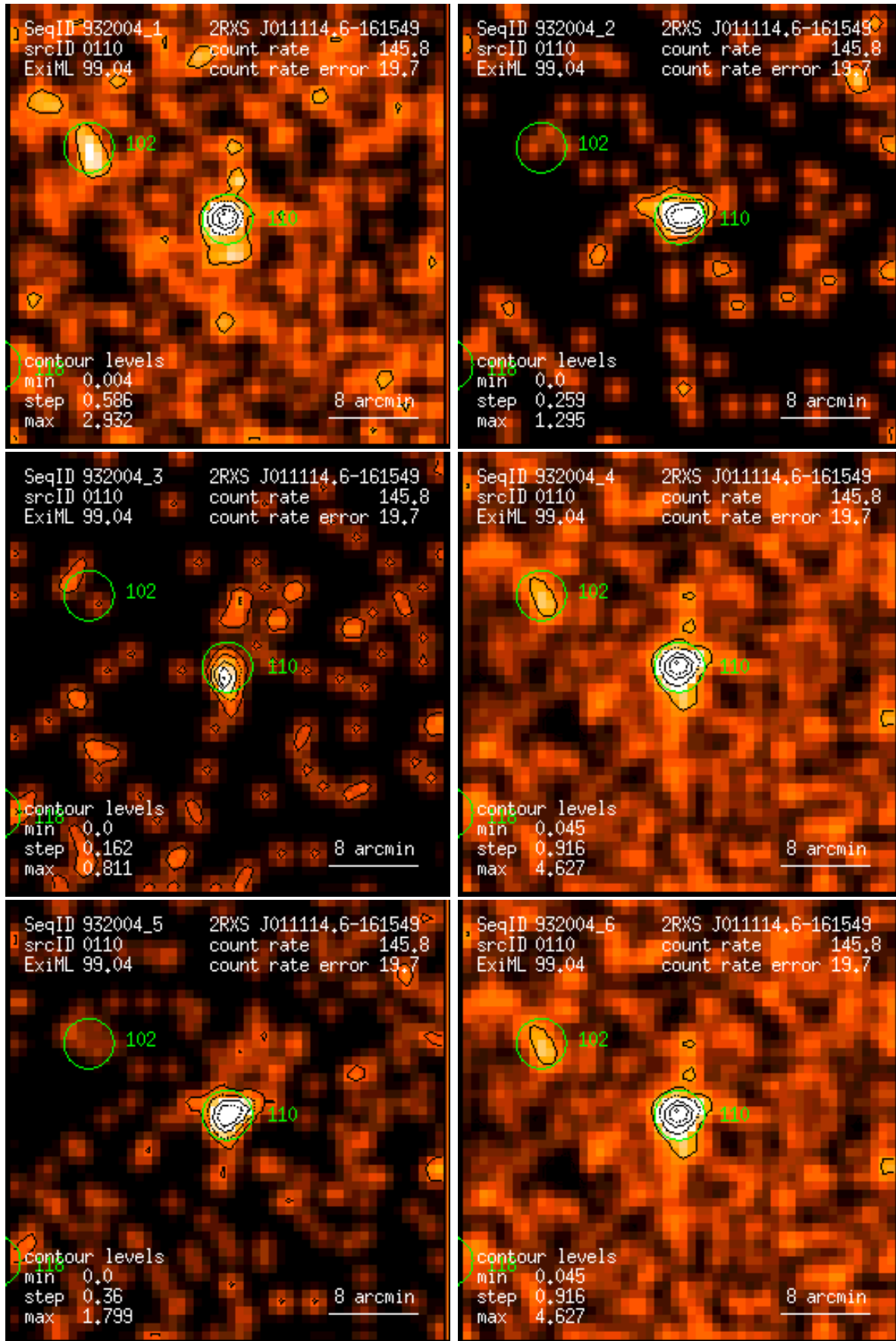
Figure 110: RASS 932004: detection 0110: band rate images, Gaussian filter: (1) PSPC channels 11 – 41, (2) 52 – 90, (3) 91 – 201, (4) 11 – 235, (5) 52 – 201, (6) 11 – 201. Broad band rates in counts/ks. Band rate contour levels in counts/ks/arcmin 2 .
