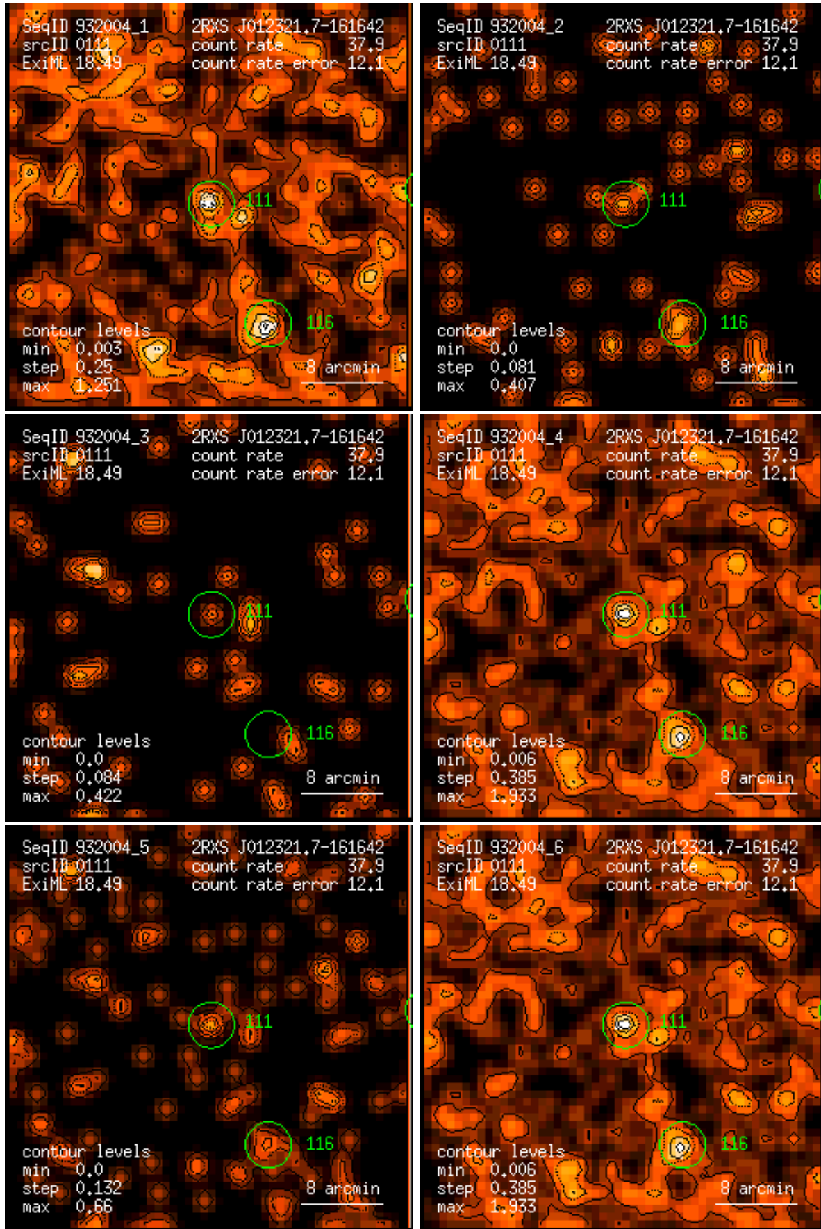
Figure 111: RASS 932004: detection 0111: band rate images, Gaussian filter: (1) PSPC channels 11 – 41, (2) 52 – 90, (3) 91 – 201, (4) 11 – 235, (5) 52 – 201, (6) 11 – 201. Broad band rates in counts/ks. Band rate contour levels in counts/ks/arcmin 2 .
