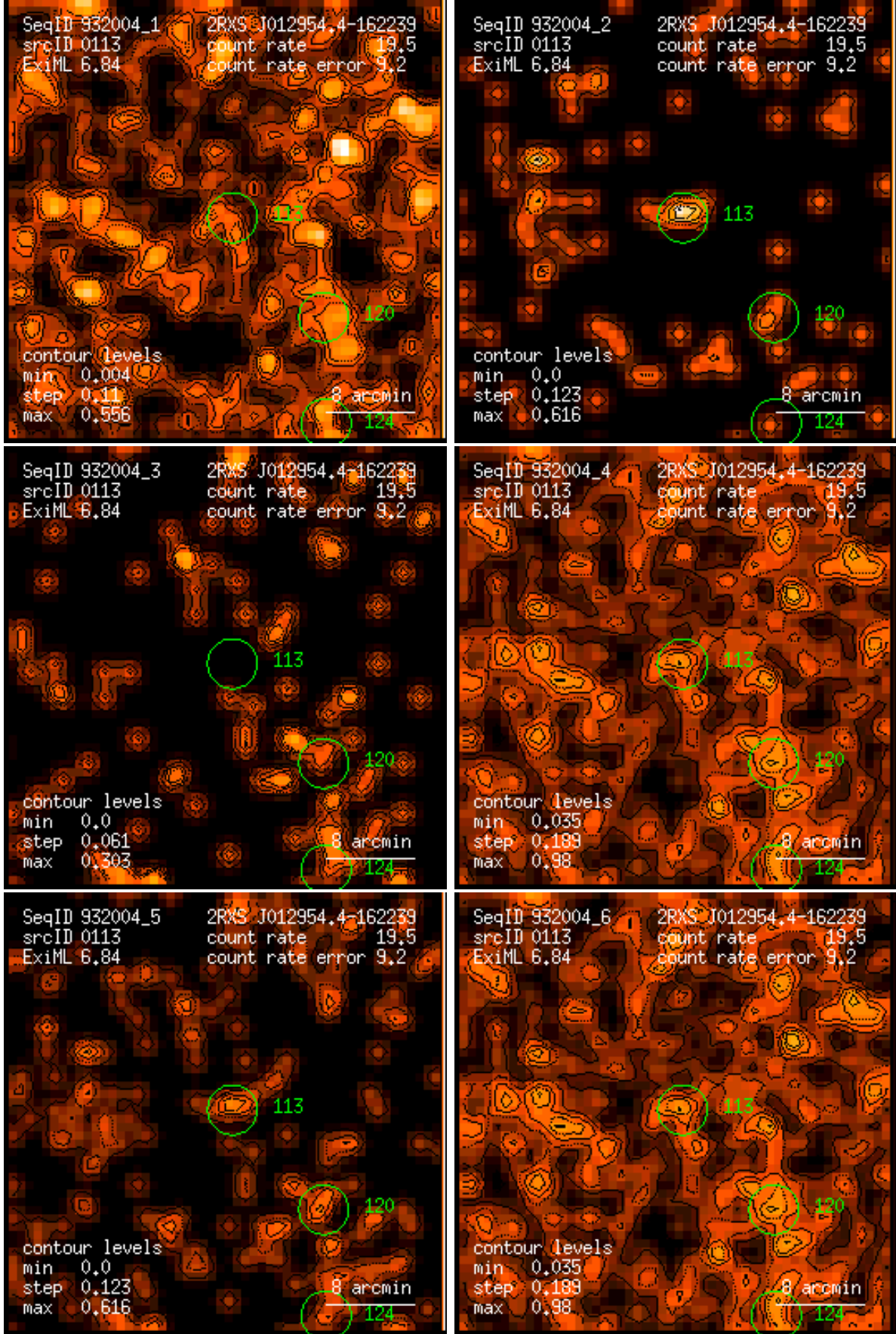
Figure 113: RASS 932004: detection 0113: band rate images, Gaussian filter: (1) PSPC channels 11 – 41, (2) 52 – 90, (3) 91 – 201, (4) 11 – 235, (5) 52 – 201, (6) 11 – 201. Broad band rates in counts/ks. Band rate contour levels in counts/ks/arcmin 2 .
