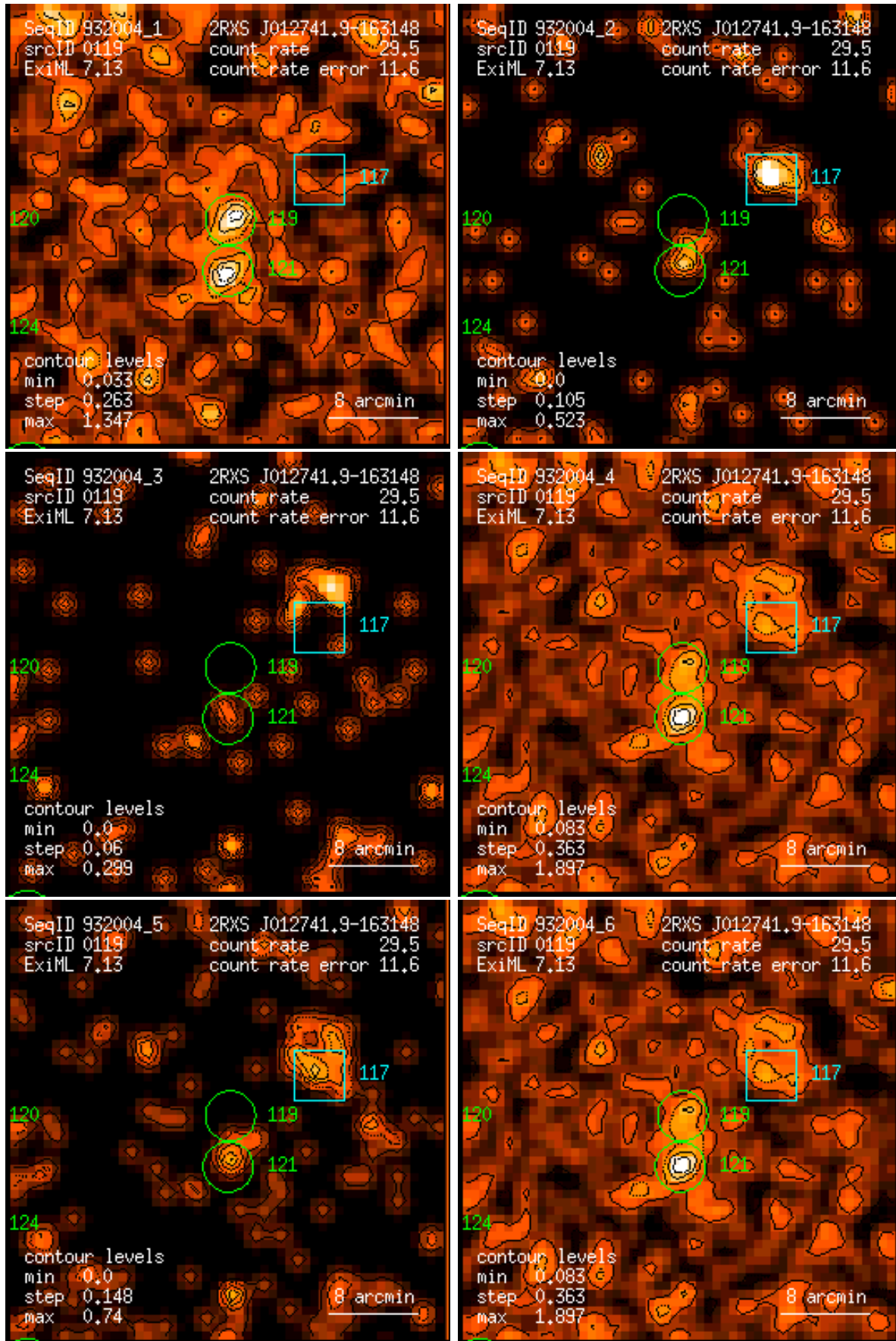
Figure 119: RASS 932004: detection 0119: band rate images, Gaussian filter: (1) PSPC channels 11 – 41, (2) 52 – 90, (3) 91 – 201, (4) 11 – 235, (5) 52 – 201, (6) 11 – 201. Broad band rates in counts/ks. Band rate contour levels in counts/ks/arcmin 2 .
