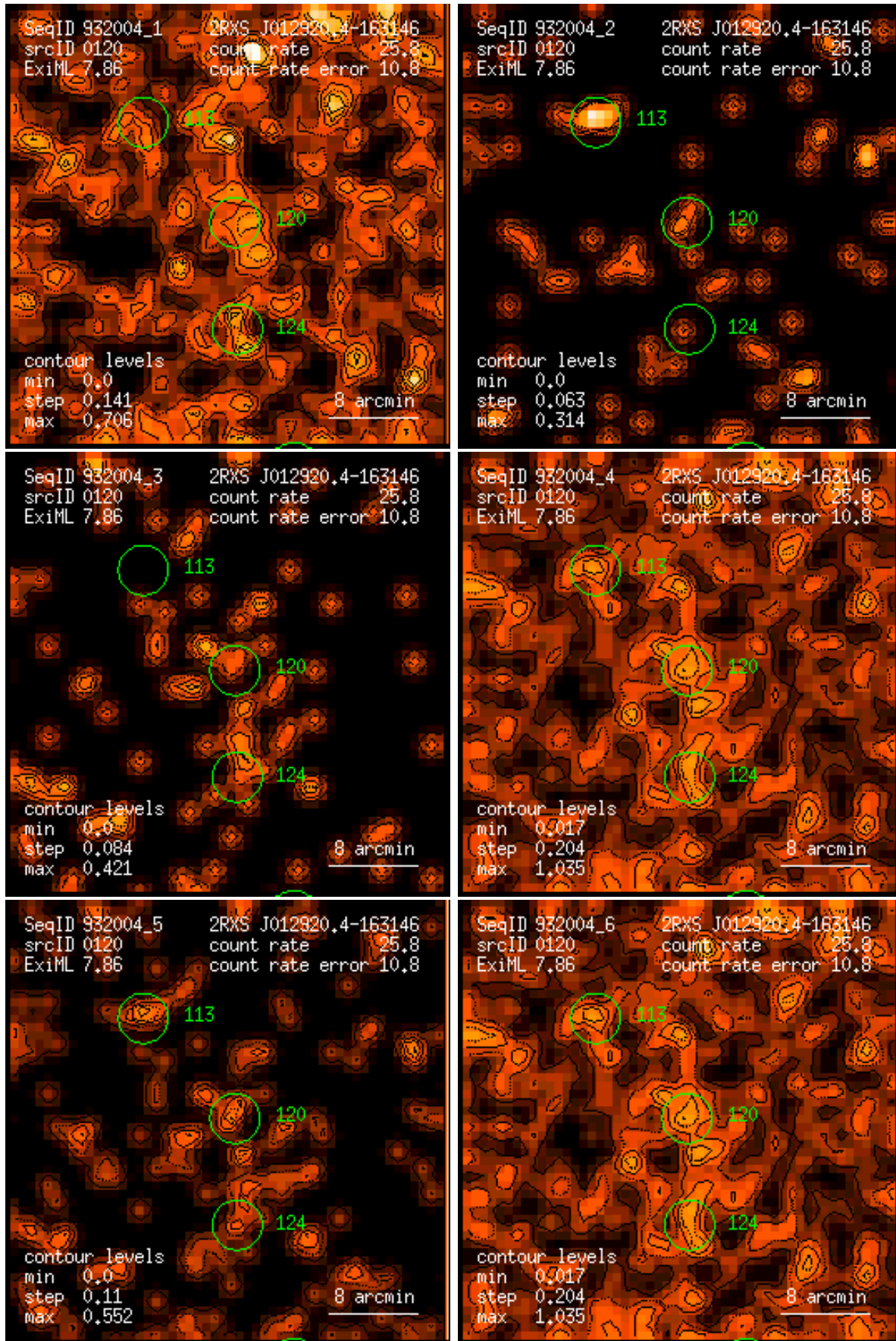
Figure 120: RASS 932004: detection 0120: band rate images, Gaussian filter: (1) PSPC channels 11 – 41, (2) 52 – 90, (3) 91 – 201, (4) 11 – 235, (5) 52 – 201, (6) 11 – 201. Broad band rates in counts/ks. Band rate contour levels in counts/ks/arcmin 2 .
