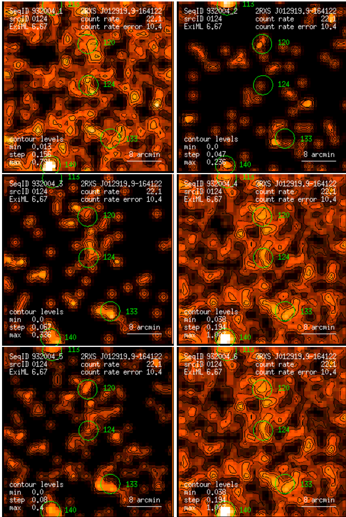
Figure 124: RASS 932004: detection 0124: band rate images, Gaussian filter: (1) PSPC channels 11 – 41, (2) 52 – 90, (3) 91 – 201, (4) 11 – 235, (5) 52 – 201, (6) 11 – 201. Broad band rates in counts/ks. Band rate contour levels in counts/ks/arcmin 2 .
