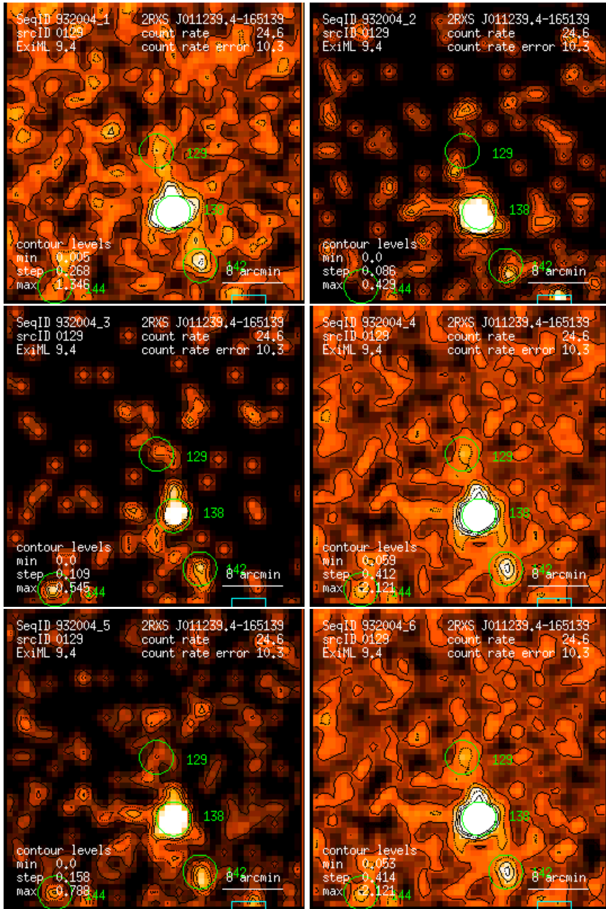
Figure 129: RASS 932004: detection 0129: band rate images, Gaussian filter: (1) PSPC channels 11 – 41, (2) 52 – 90, (3) 91 – 201, (4) 11 – 235, (5) 52 – 201, (6) 11 – 201. Broad band rates in counts/ks. Band rate contour levels in counts/ks/arcmin 2 .
