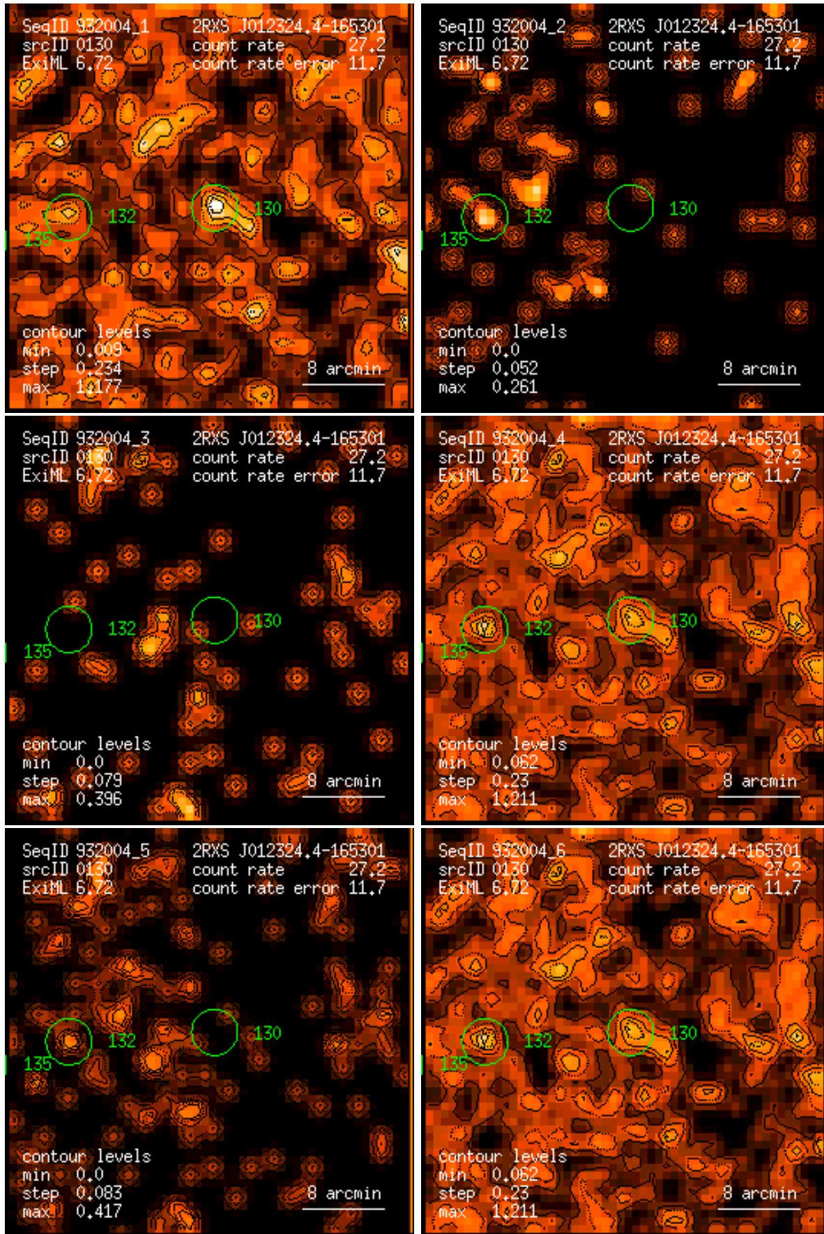
Figure 130: RASS 932004: detection 0130: band rate images, Gaussian filter: (1) PSPC channels 11 – 41, (2) 52 – 90, (3) 91 – 201, (4) 11 – 235, (5) 52 – 201, (6) 11 – 201. Broad band rates in counts/ks. Band rate contour levels in counts/ks/arcmin 2 .
