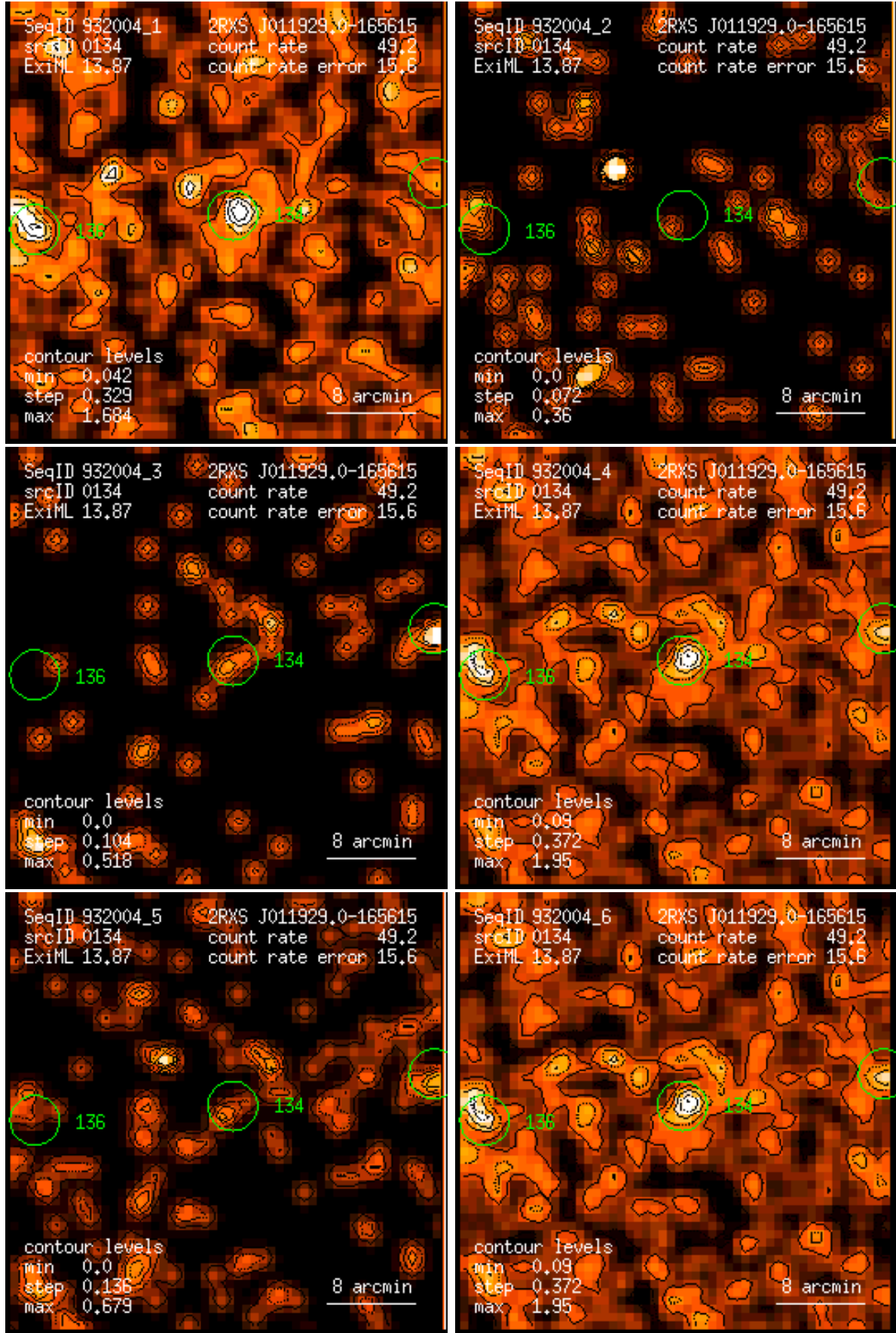
Figure 134: RASS 932004: detection 0134: band rate images, Gaussian filter: (1) PSPC channels 11 – 41, (2) 52 – 90, (3) 91 – 201, (4) 11 – 235, (5) 52 – 201, (6) 11 – 201. Broad band rates in counts/ks. Band rate contour levels in counts/ks/arcmin 2 .
