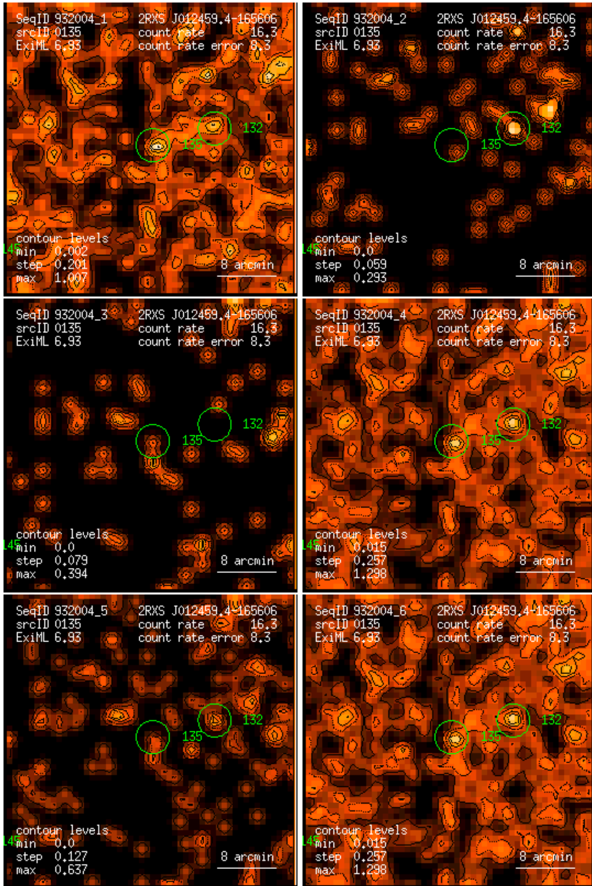
Figure 135: RASS 932004: detection 0135: band rate images, Gaussian filter: (1) PSPC channels 11 – 41, (2) 52 – 90, (3) 91 – 201, (4) 11 – 235, (5) 52 – 201, (6) 11 – 201. Broad band rates in counts/ks. Band rate contour levels in counts/ks/arcmin 2 .
