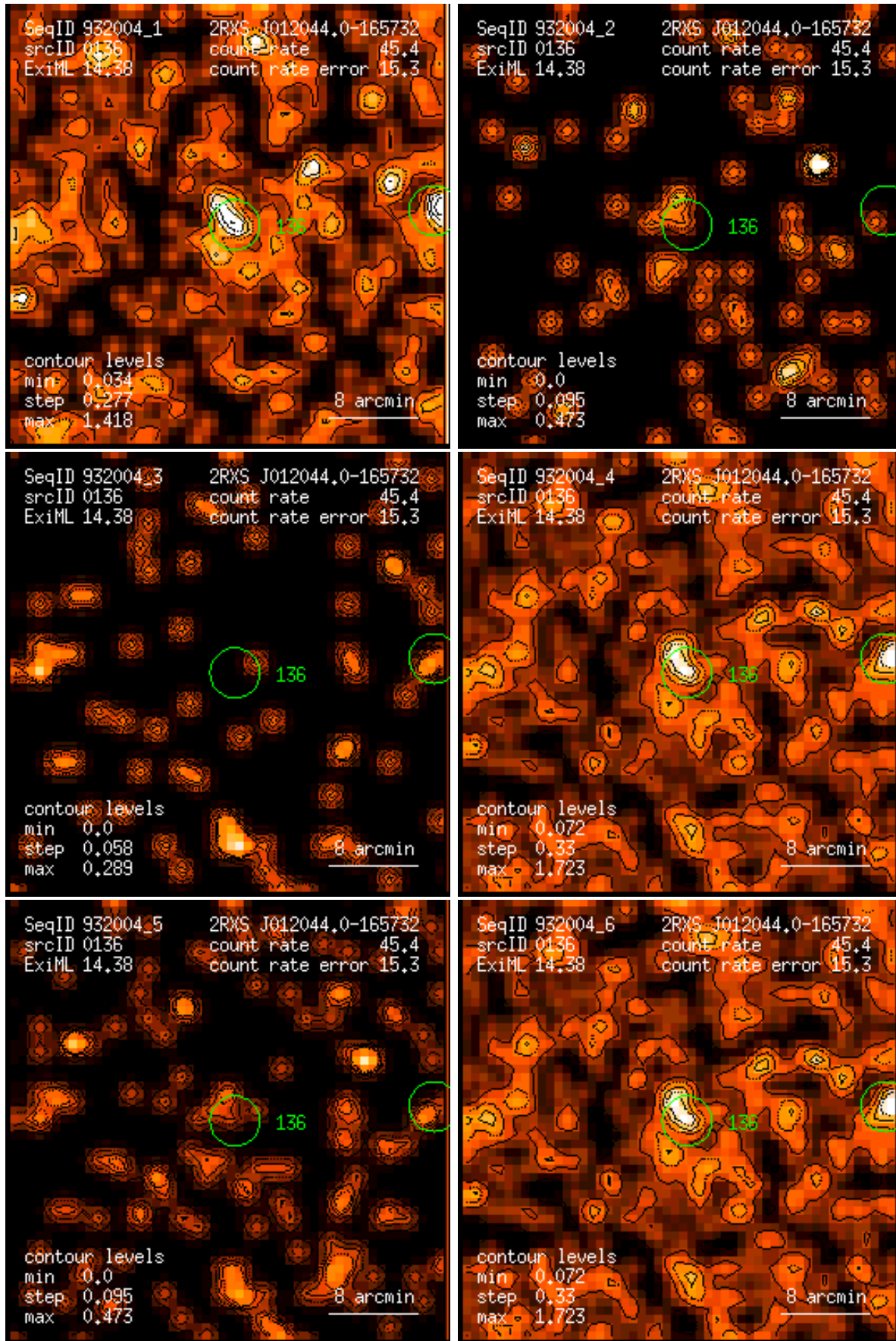
Figure 136: RASS 932004: detection 0136: band rate images, Gaussian filter: (1) PSPC channels 11 – 41, (2) 52 – 90, (3) 91 – 201, (4) 11 – 235, (5) 52 – 201, (6) 11 – 201. Broad band rates in counts/ks. Band rate contour levels in counts/ks/arcmin 2 .
