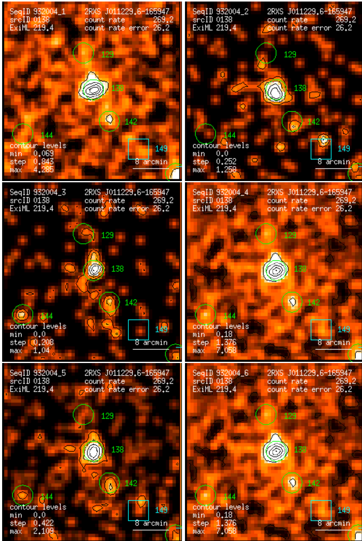
Figure 138: RASS 932004: detection 0138: band rate images, Gaussian filter: (1) PSPC channels 11 – 41, (2) 52 – 90, (3) 91 – 201, (4) 11 – 235, (5) 52 – 201, (6) 11 – 201. Broad band rates in counts/ks. Band rate contour levels in counts/ks/arcmin 2 .
