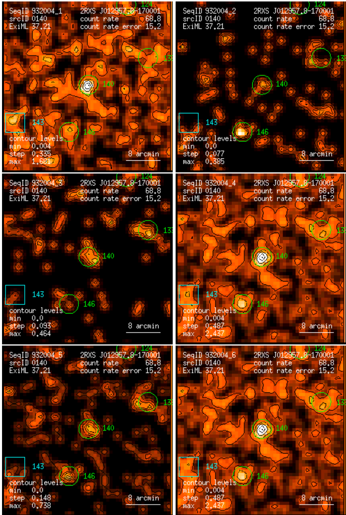
Figure 140: RASS 932004: detection 0140: band rate images, Gaussian filter: (1) PSPC channels 11 – 41, (2) 52 – 90, (3) 91 – 201, (4) 11 – 235, (5) 52 – 201, (6) 11 – 201. Broad band rates in counts/ks. Band rate contour levels in counts/ks/arcmin 2 .
