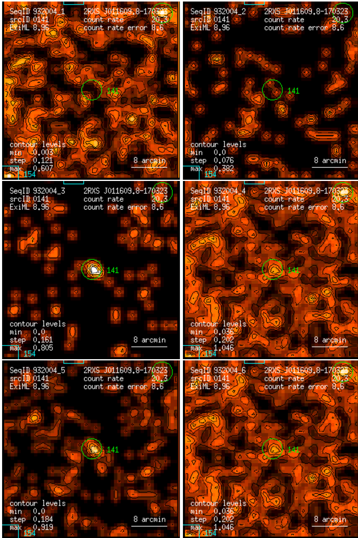
Figure 141: RASS 932004: detection 0141: band rate images, Gaussian filter: (1) PSPC channels 11 – 41, (2) 52 – 90, (3) 91 – 201, (4) 11 – 235, (5) 52 – 201, (6) 11 – 201. Broad band rates in counts/ks. Band rate contour levels in counts/ks/arcmin 2 .
