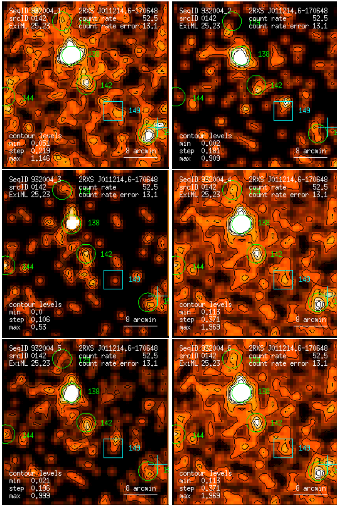
Figure 142: RASS 932004: detection 0142: band rate images, Gaussian filter: (1) PSPC channels 11 – 41, (2) 52 – 90, (3) 91 – 201, (4) 11 – 235, (5) 52 – 201, (6) 11 – 201. Broad band rates in counts/ks. Band rate contour levels in counts/ks/arcmin 2 .
